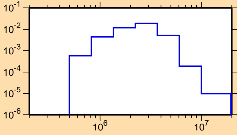
\sigma vs. E for ^{83}\text{Se}(n,n_4)
