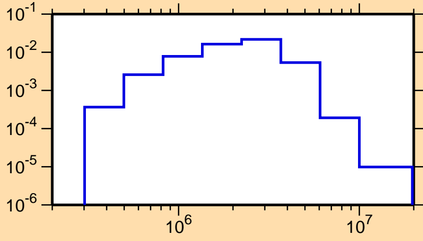
\sigma vs. E for ^{83}\text{Se}(n,n_2)
