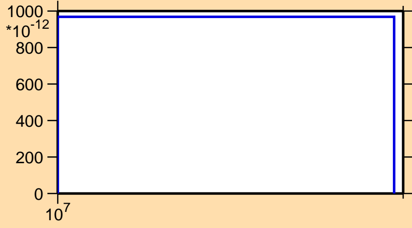
\sigma vs. E for ^{83}\text{Se}(n,nd)
