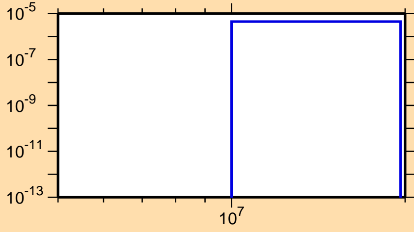
\sigma vs. E for ^{83}\text{Se}(n,\alpha)
