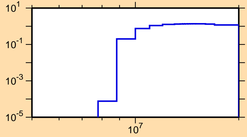
\sigma vs. E for ^{84}\text{Se}(n,2n)
