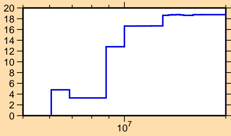
\Delta\sigma/\sigma vs. E for ^{84}\text{Se}(n,n\text{cont.})
