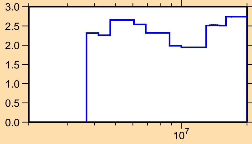
\Delta\sigma/\sigma vs. E for ^{84}\text{Se}(n,n\text{onel.})
