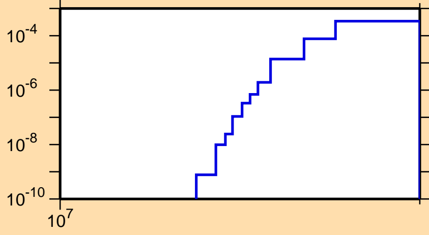
\sigma vs. E for ^{84}\text{Se}(n,d)
