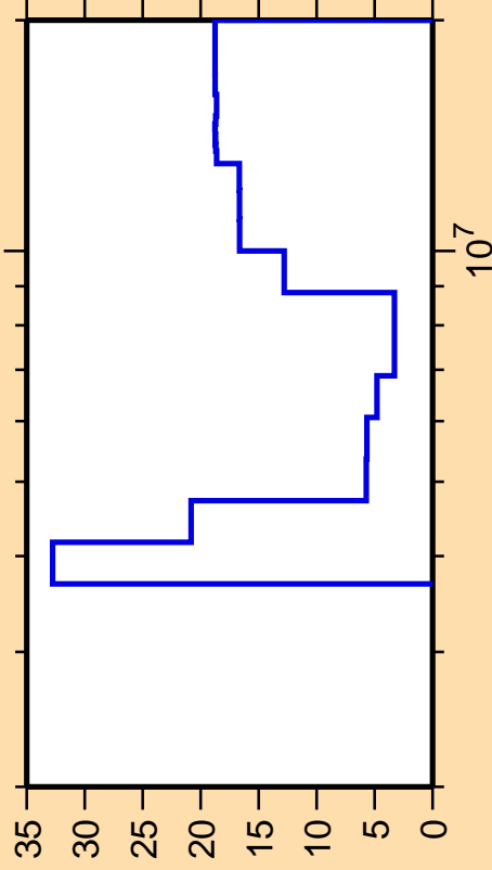
\Delta\sigma/\sigma vs. E for ^{84}\text{Se}(n,n\text{cont.})
