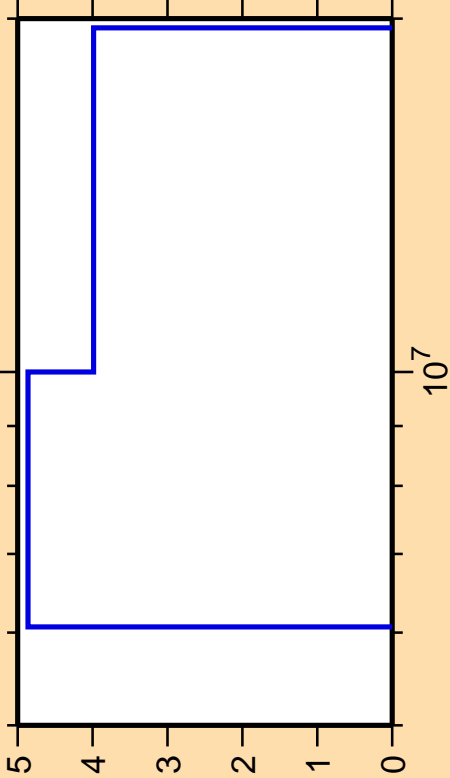
\Delta\sigma/\sigma vs. E for ^{84}\text{Se}(n,2n)
