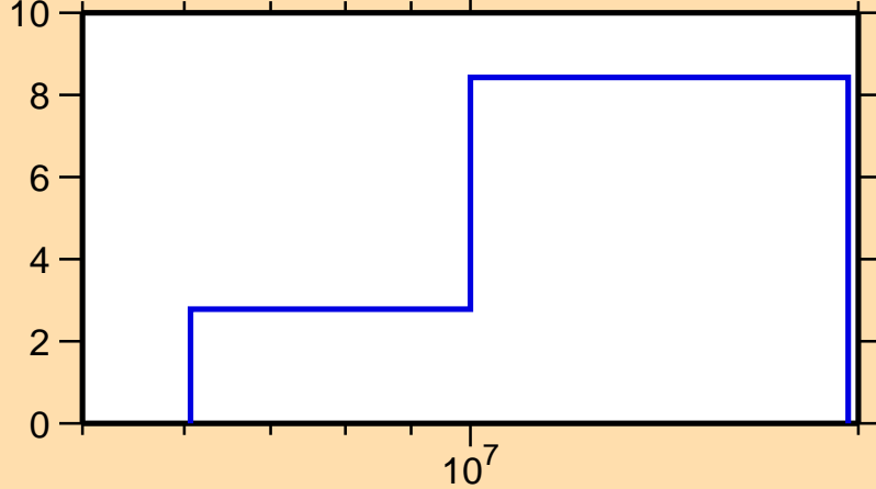
\Delta\sigma/\sigma vs. E for ^{84}\text{Se}(n,\text{el.})
