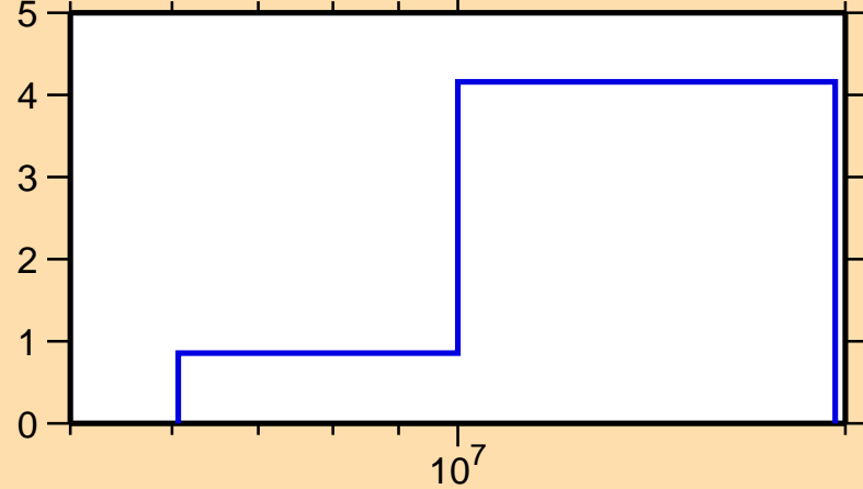
\Delta\sigma/\sigma vs. E for ^{84}\text{Se}(n,\text{tot.})
