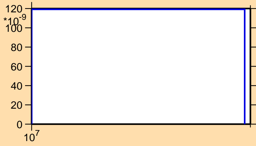
\sigma vs. E for ^{84}\text{Se}(n,t)
