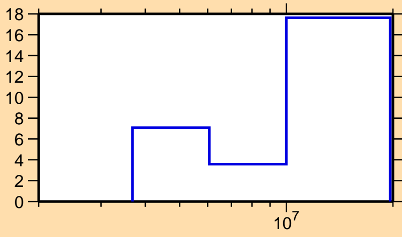
\Delta\sigma/\sigma vs. E for ^{84}\text{Se}(n,ncont.)
