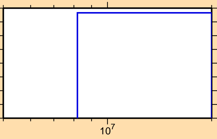
\sigma vs. E for ^{84}\text{Se}(n,d)
