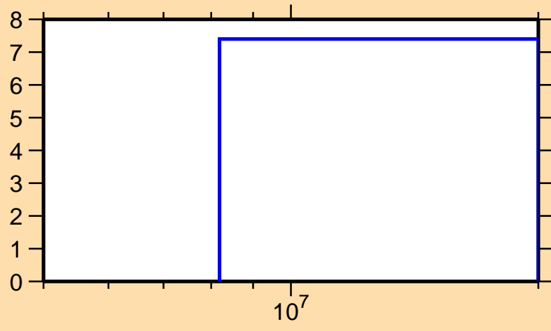
\Delta\sigma/\sigma vs. E for ^{84}\text{Se}(n,el.)
