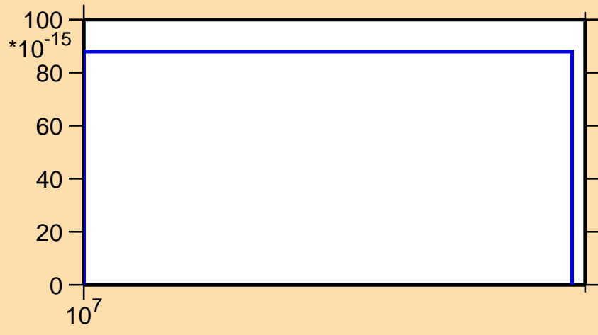
\sigma vs. E for ^{85}\text{Se}(n,2np)
