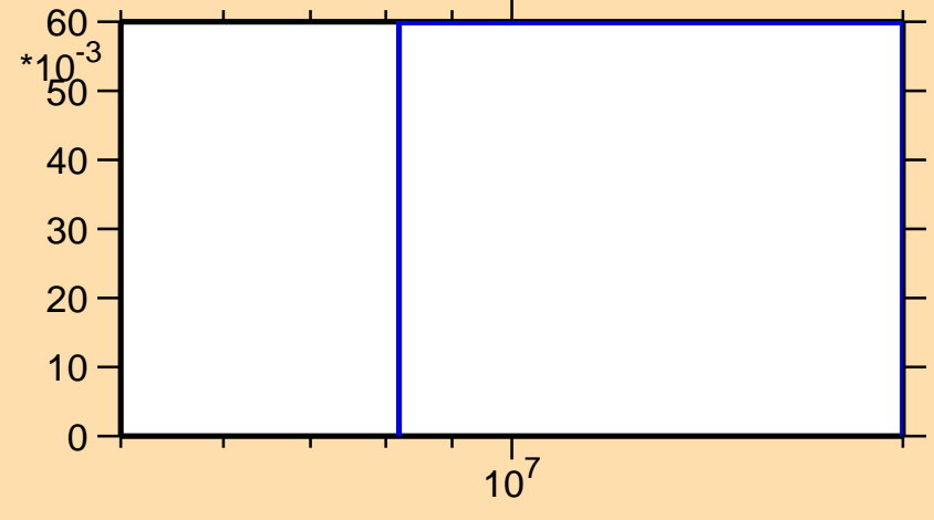
\sigma vs. E for ^{85}\text{Se}(n,3n)
