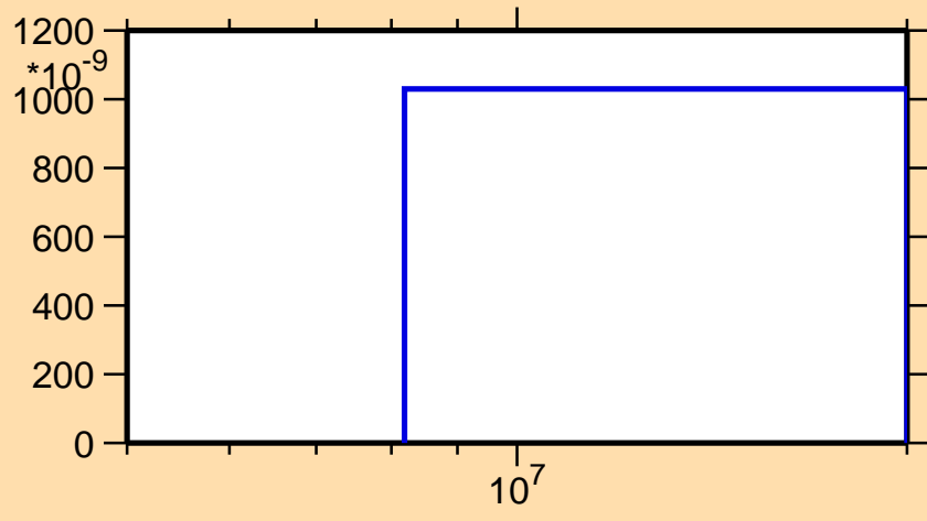
\sigma vs. E for ^{85}\text{Se}(n,n\alpha)
