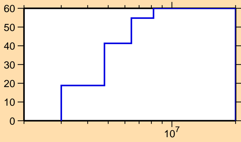
\Delta\sigma/\sigma vs. E for ^{85}\text{Se}(n,n\text{cont.})
