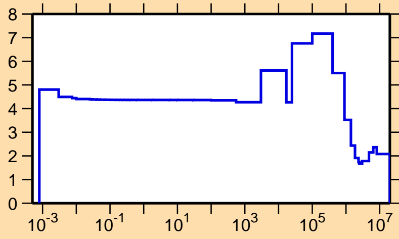
\sigma vs. E for ^{85}\text{Se}(n,\text{el.})
