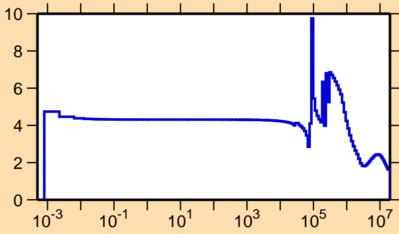
\sigma vs. E for ^{86}\text{Se}(n,\text{el.})
