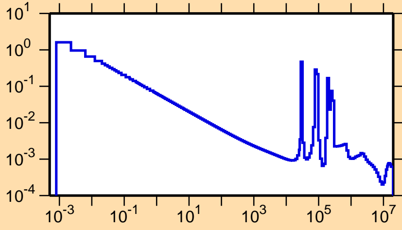
\sigma vs. E for ^{86}\text{Se}(n,\gamma)
