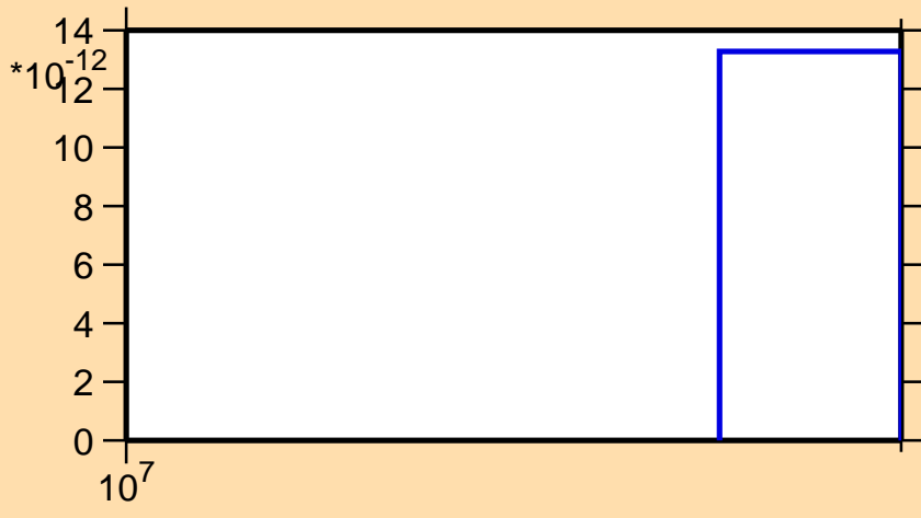
\sigma vs. E for ^{86}\text{Se}(n,nd)
