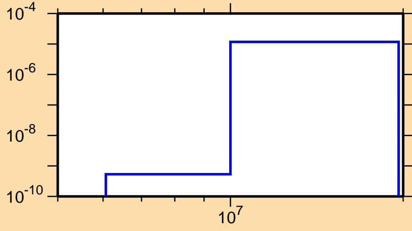
\sigma vs. E for ^{86}\text{Se}(n,\alpha)
