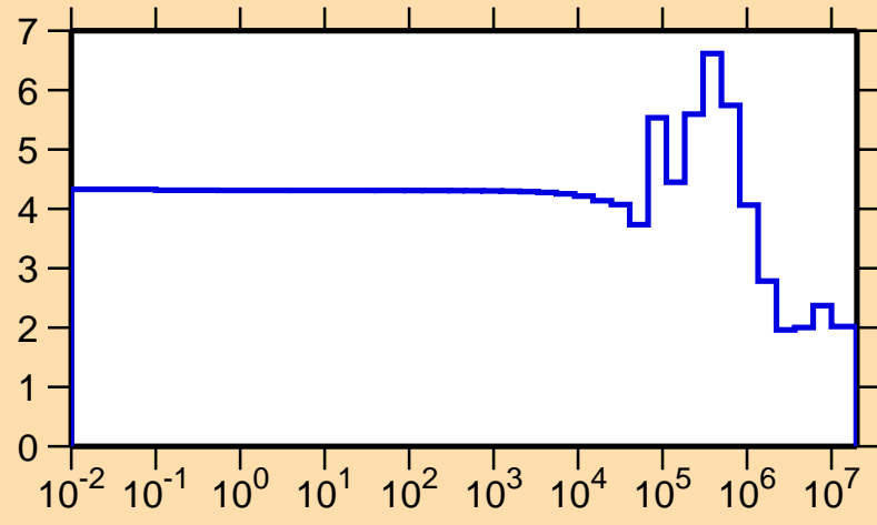
\sigma vs. E for ^{86}\text{Se}(n,\text{el.})
