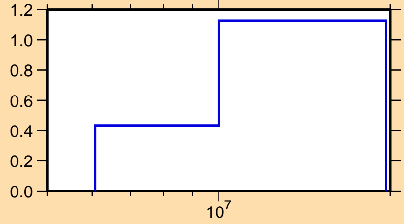
\sigma vs. E for ^{86}\text{Se}(n,2n)
