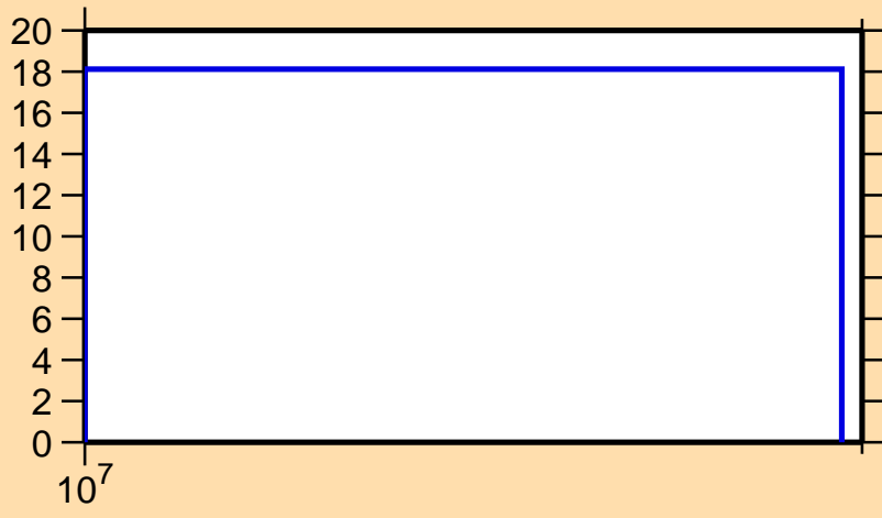
\Delta\sigma/\sigma vs. E for ^{86}\text{Se}(n,el.)
