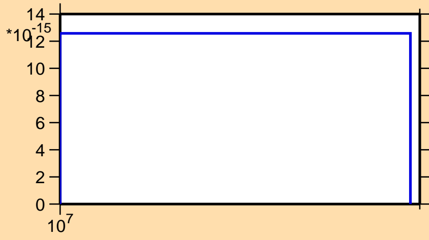
\sigma vs. E for ^{86}\text{Se}(n,2n\alpha)
