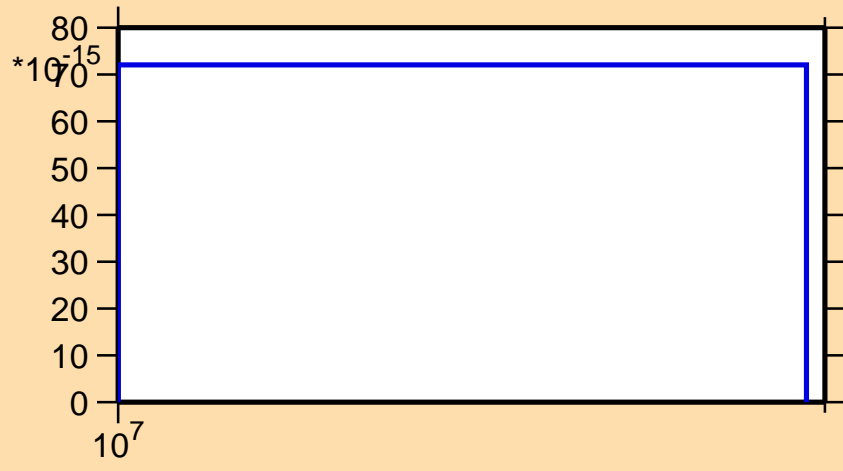
\sigma vs. E for ^{86}\text{Se}(n,nd)
