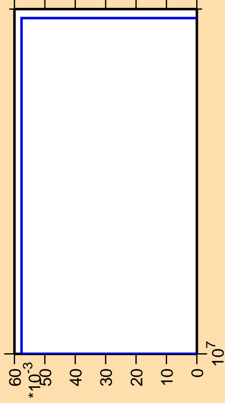
\Delta\sigma/\sigma vs. E for ^{86}\text{Se}(n,nd)
