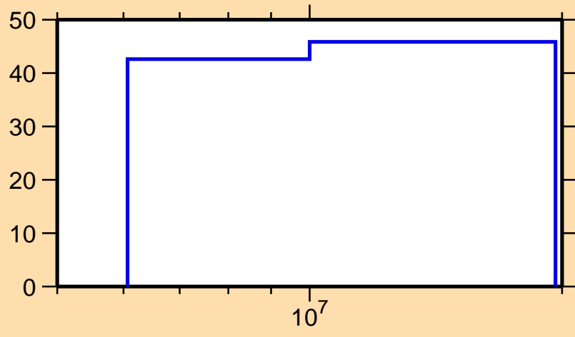
\Delta\sigma/\sigma vs. E for ^{86}\text{Se}(n,n_1)
