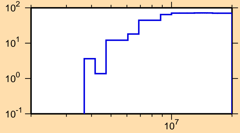
\Delta\sigma/\sigma vs. E for ^{87}\text{Se}(n,\text{inel.})
