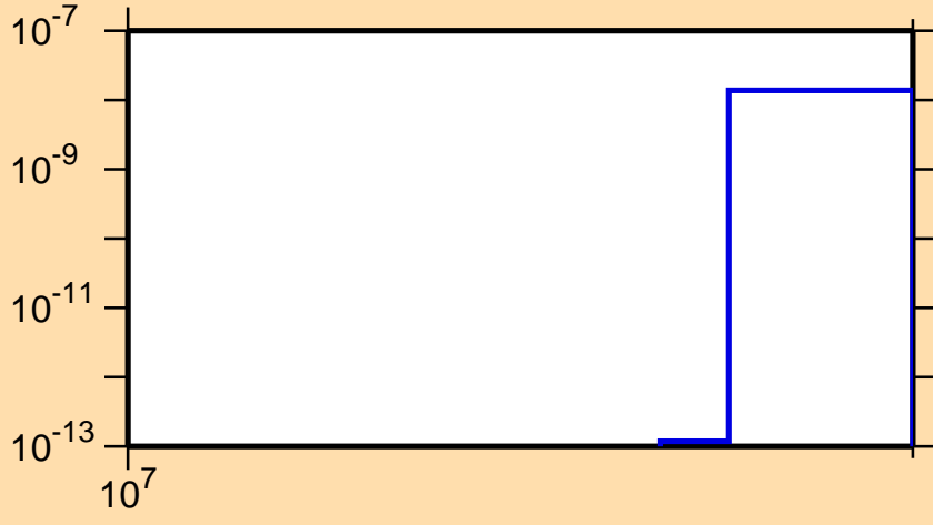
\sigma vs. E for ^{87}\text{Se}(n,nd)
