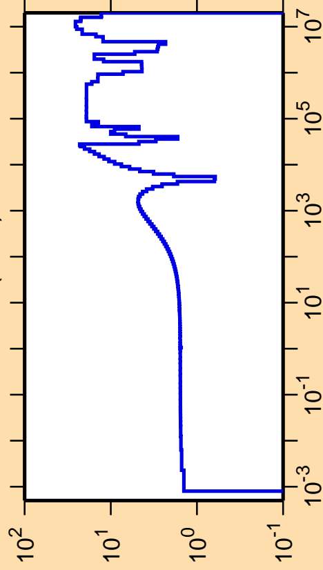
\Delta\sigma/\sigma vs. E for ^{87}\text{Se}(n,\text{el.})
