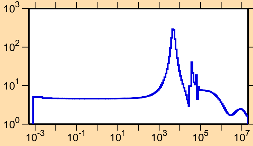
\sigma vs. E for ^{87}\text{Se}(n,\text{el.})
