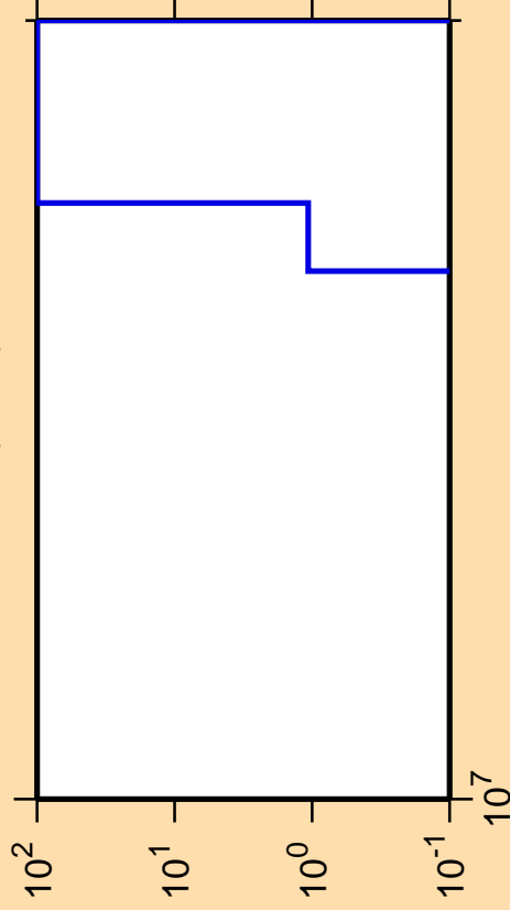
\Delta\sigma/\sigma vs. E for ^{87}\text{Se}(n,nd)
