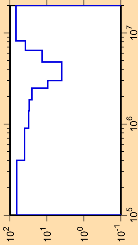
\Delta\sigma/\sigma vs. E for ^{87}\text{Se}(n,n\text{cont.})
