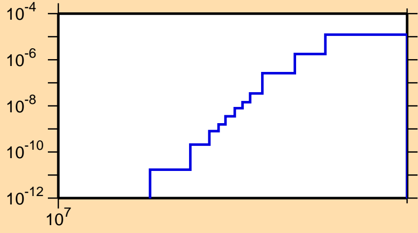
\sigma vs. E for ^{88}\text{Se}(n,n\alpha)
