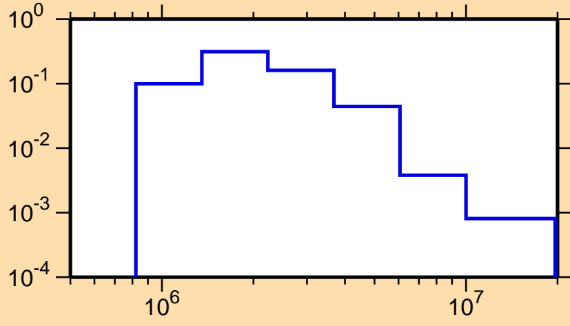
\sigma vs. E for ^{88}\text{Se}(n,n_2)
