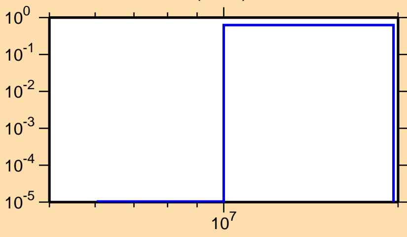
\sigma vs. E for ^{88}\text{Se}(n,3n)
