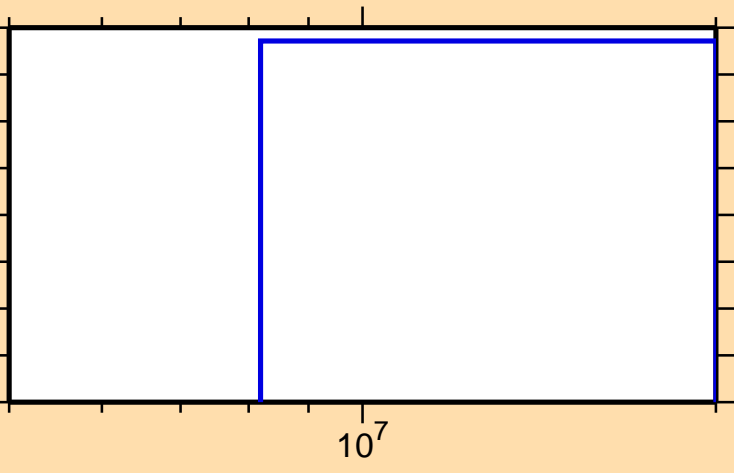
\sigma vs. E for ^{88}\text{Se}(n,nt)
