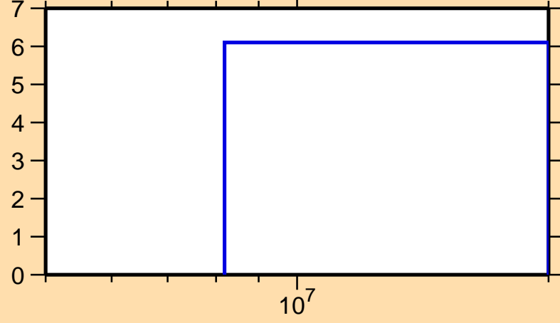
\Delta\sigma/\sigma vs. E for ^{88}\text{Se}(n,\text{nonel.})
