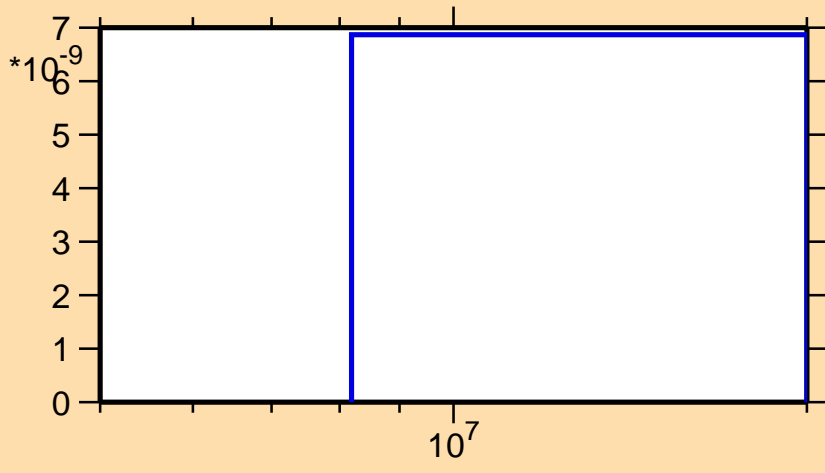
\sigma vs. E for ^{88}\text{Se}(n,np)
