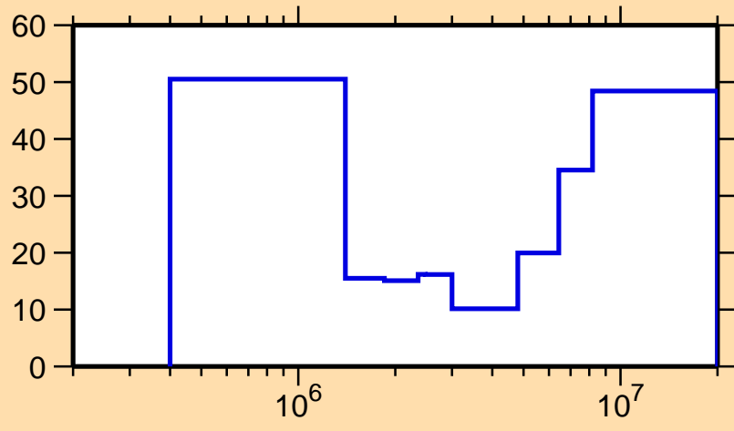
\Delta\sigma/\sigma vs. E for ^{88}\text{Se}(n,\text{inel.})
