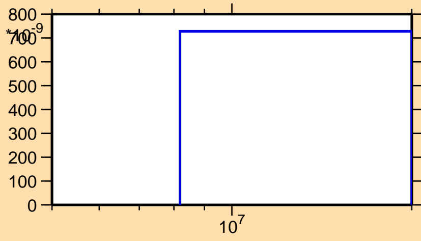
\sigma vs. E for ^{88}\text{Se}(n,t)
