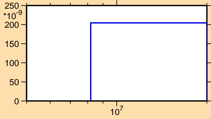
\sigma vs. E for ^{88}\text{Se}(n,n\alpha)
