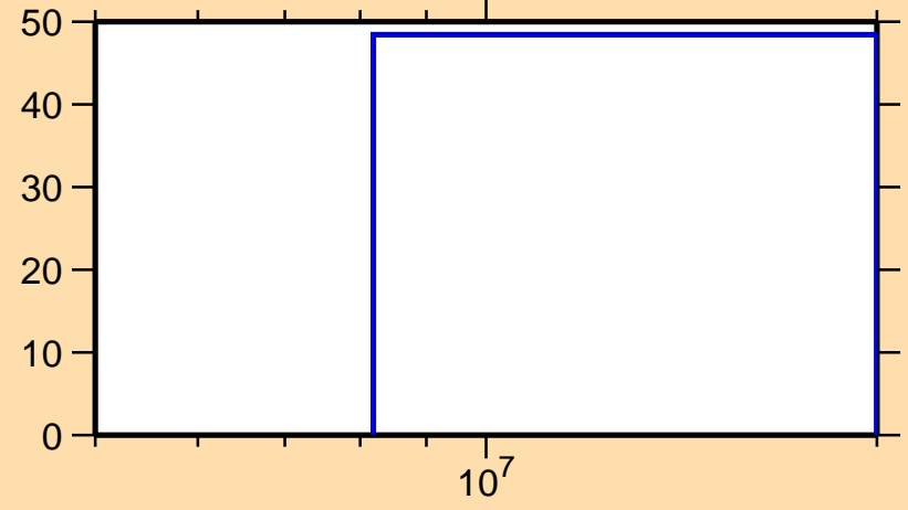
\Delta\sigma/\sigma vs. E for ^{88}\text{Se}(n,inel.)
