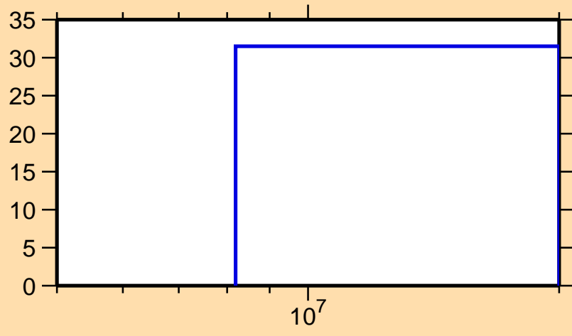
\Delta\sigma/\sigma vs. E for ^{88}\text{Se}(n,2n)
