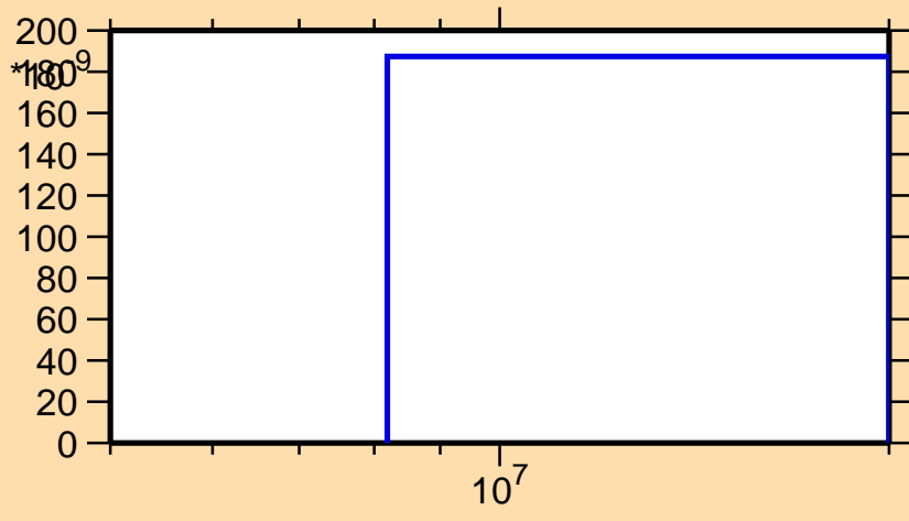
\sigma vs. E for ^{88}\text{Se}(n,d)
