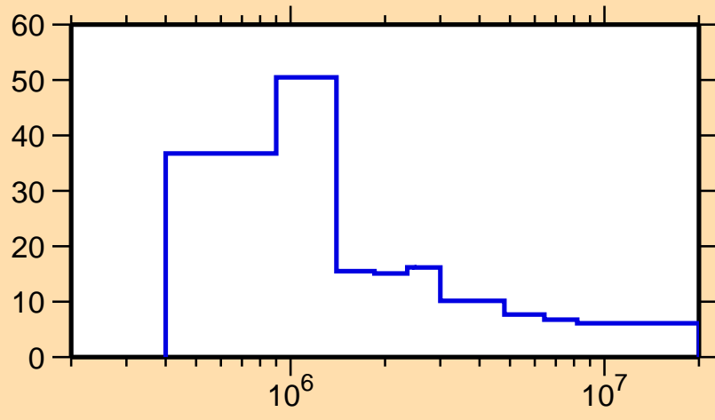
\Delta\sigma/\sigma vs. E for ^{88}\text{Se}(n,\text{nonel.})
