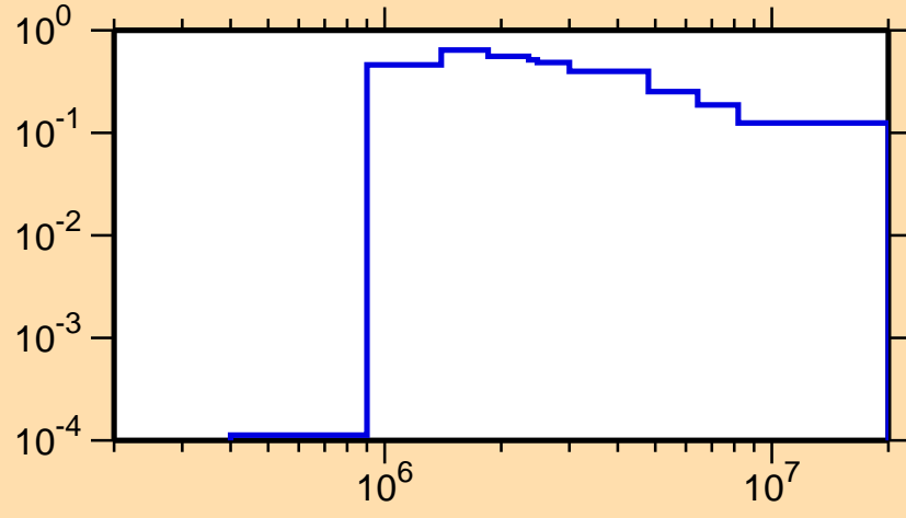
\sigma vs. E for ^{88}\text{Se}(n,n_1)
