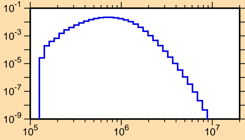
\sigma vs. E for ^{265}_3 )
