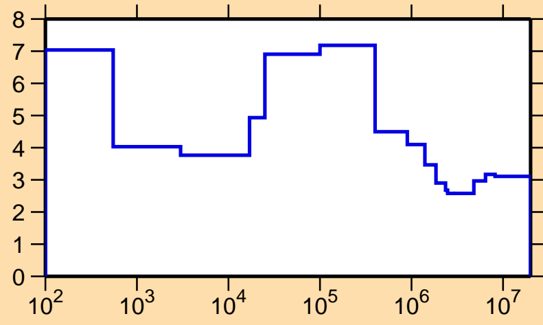
\sigma vs. E for ^{265}
