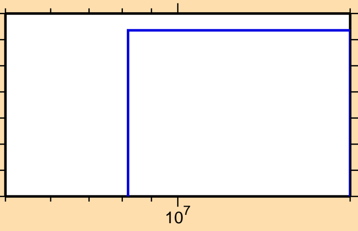
\sigma vs. E for ^{268}
