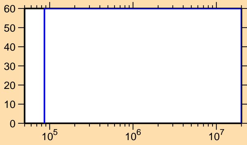
\Delta\sigma/\sigma vs. E for ^{269}\text{Tc}
