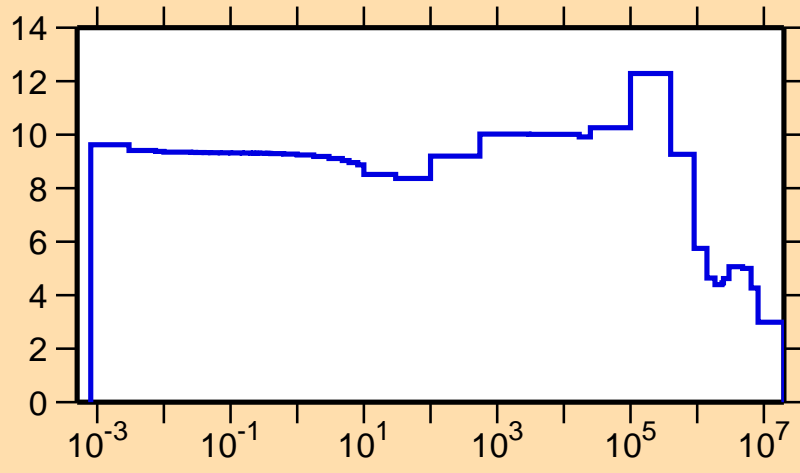
\sigma vs. E for ^{269}
