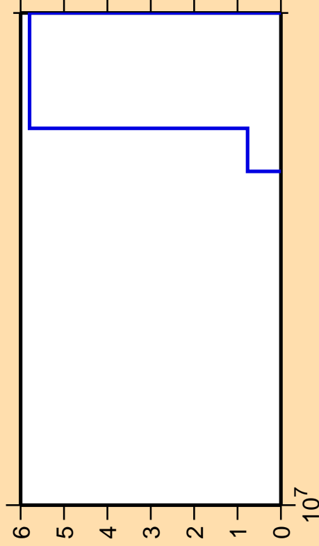
\Delta\sigma/\sigma vs. E for ^{271}\text{He3}
