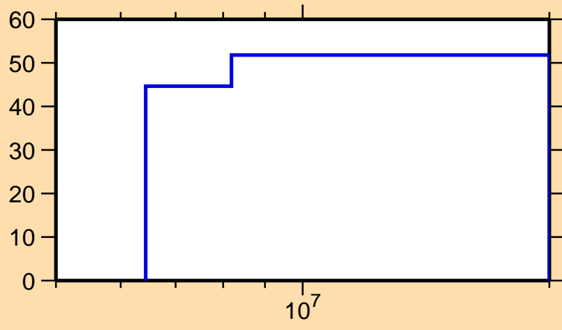
\Delta\sigma/\sigma vs. E for ^{272}\text{Po}
