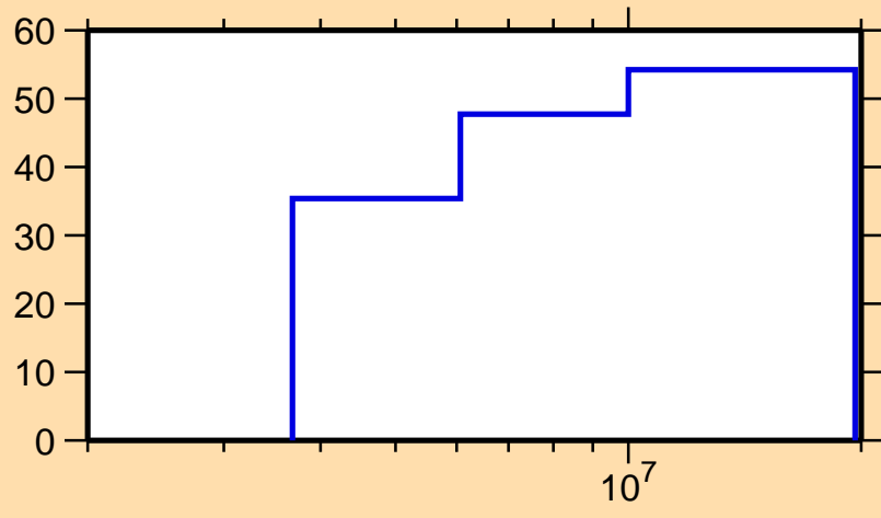
\Delta\sigma/\sigma vs. E for ^{273}_1
