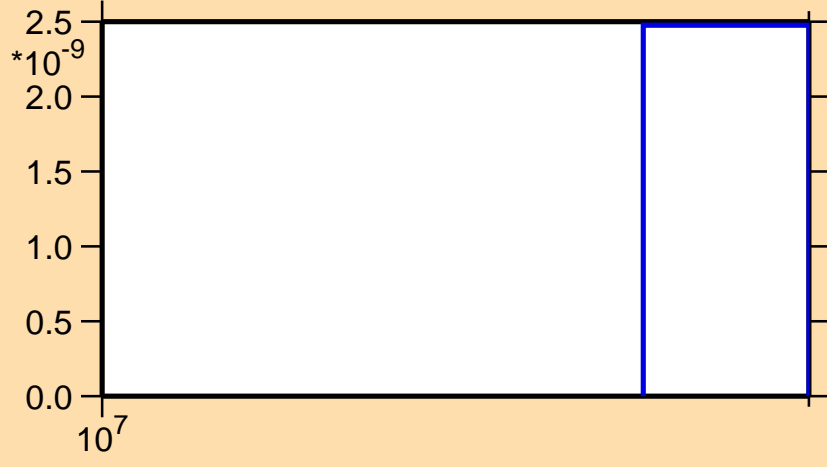
\sigma vs. E for ^{26}\text{Si} (mt 34)
