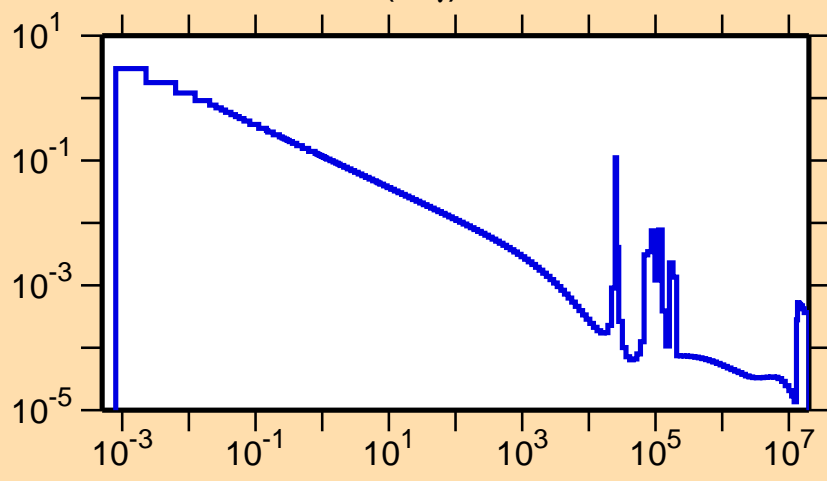
\sigma vs. E for ^{26}\text{Si}(n,\gamma)
