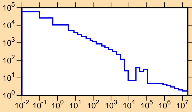
\sigma vs. E for ^{27}\text{Si}(n,\text{tot.})
