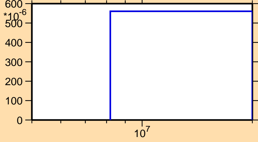
\sigma vs. E for ^{27}\text{Si}(n,\text{pd})
