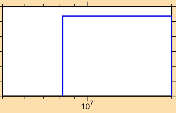
\sigma vs. E for ^{28}\text{Si}(n,\text{pd})
