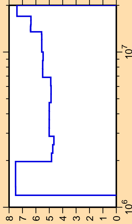
\Delta\sigma/\sigma vs. E for ^{29}\text{Si}(n,\text{nonel.})
