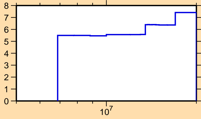
\Delta\sigma/\sigma vs. E for ^{29}\text{Si}(n,n\text{onel.})
