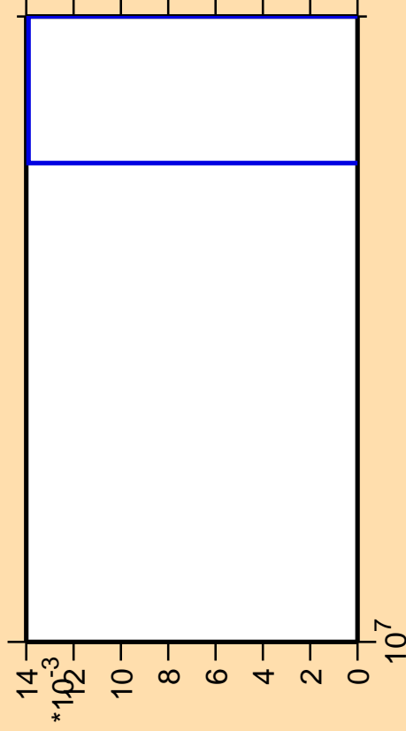
\Delta\sigma/\sigma vs. E for ^{29}\text{Si}(n,2n\alpha)
