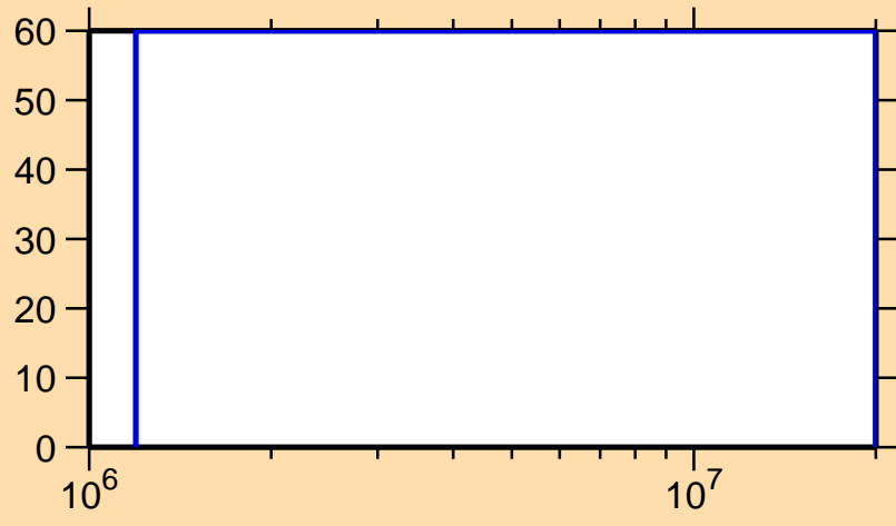
\Delta\sigma/\sigma vs. E for ^{29}\text{Si}(n,\gamma)
