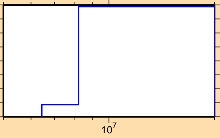
\sigma vs. E for ^{29}\text{Si}(n,n\text{cont.})
