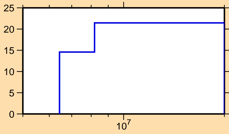
\Delta\sigma/\sigma vs. E for ^{29}\text{Si}(n,ncont.)
