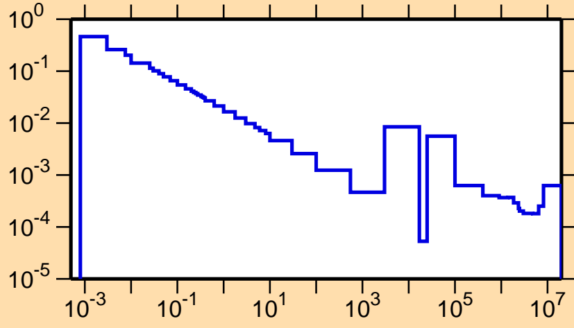
\sigma vs. E for ^{29}\text{Si}(n,\gamma)
