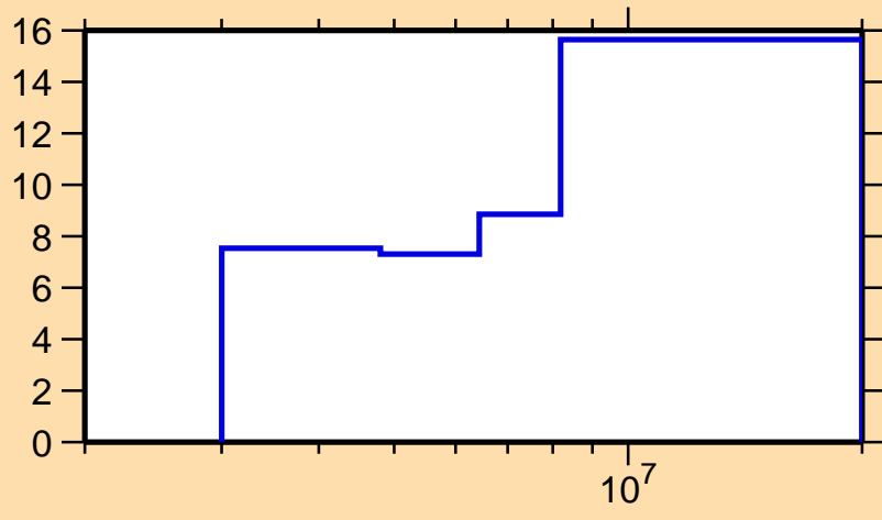
\Delta\sigma/\sigma vs. E for ^{29}\text{Si}(n,n_1)
