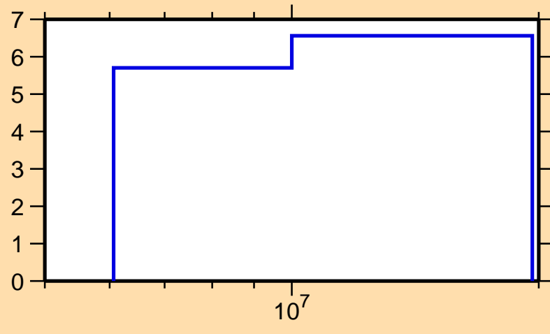
\Delta\sigma/\sigma vs. E for ^{30}\text{Si}(n,\text{nonel.})
