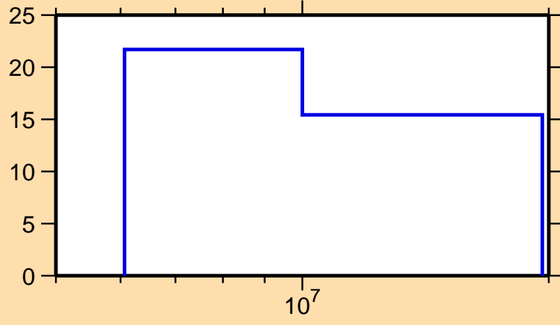
\Delta\sigma/\sigma vs. E for ^{30}\text{Si}(n,ncont.)
