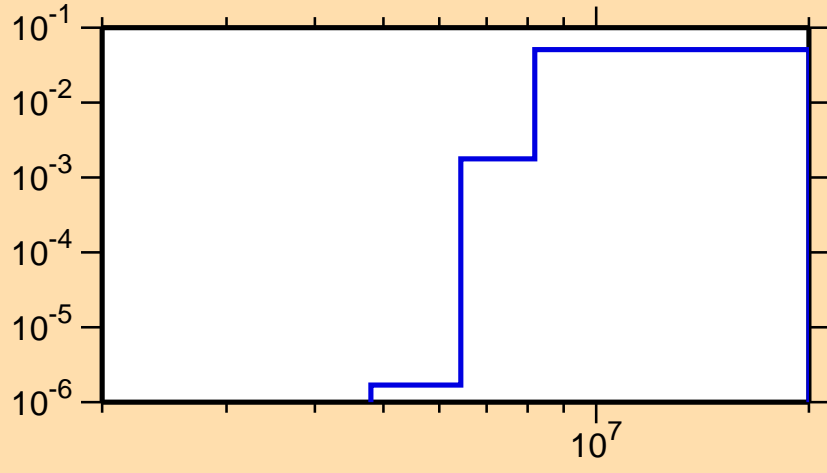
\sigma vs. E for ^{30}\text{Si}(n,\alpha)
