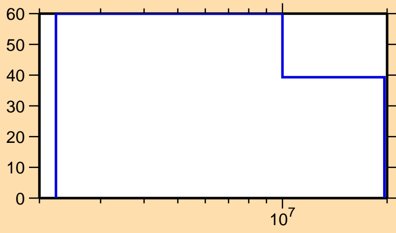
\Delta\sigma/\sigma vs. E for ^{31}\text{Si}(n,\gamma)
