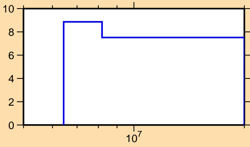
\Delta\sigma/\sigma vs. E for ^{31}\text{Si}(n,el.)
