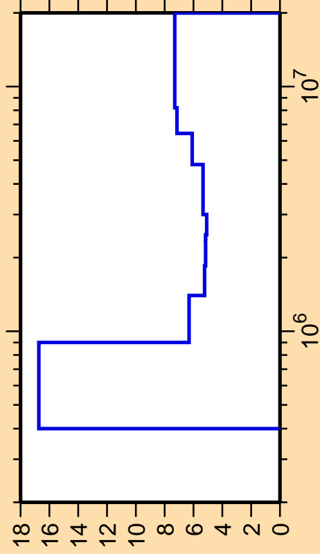
\Delta\sigma/\sigma vs. E for ^{31}\text{Si}(n,\text{nonel.})
