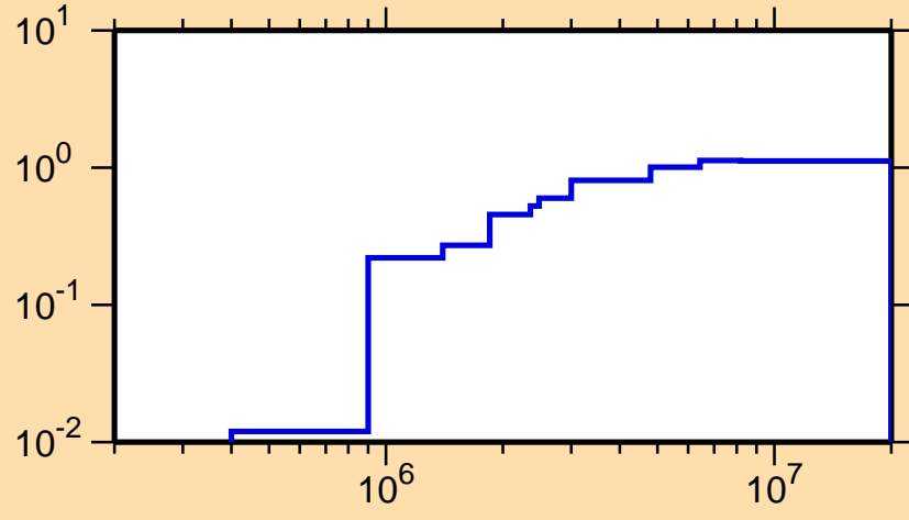
\sigma vs. E for ^{31}\text{Si}(n,\text{nonel.})
