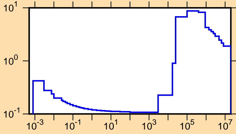
\sigma vs. E for ^{31}\text{Si}(n,\text{tot.})
