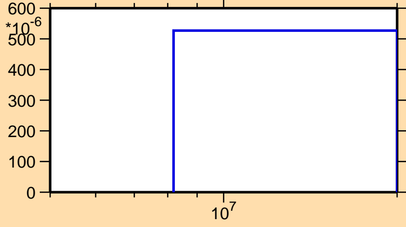
\sigma vs. E for ^{31}\text{Si}(n,n\alpha)
