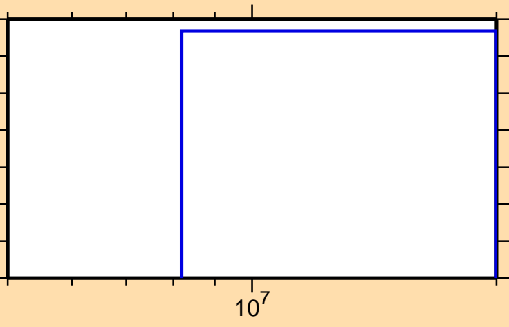
\sigma vs. E for ^{31}\text{Si}(n,t)
