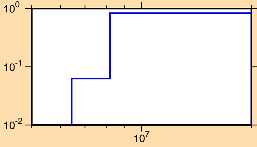
\sigma vs. E for ^{31}\text{Si}(n,2n)
