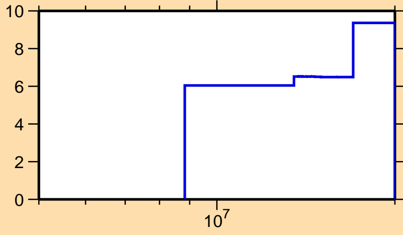
\Delta\sigma/\sigma vs. E for ^{32}\text{Si}(n,2n)
