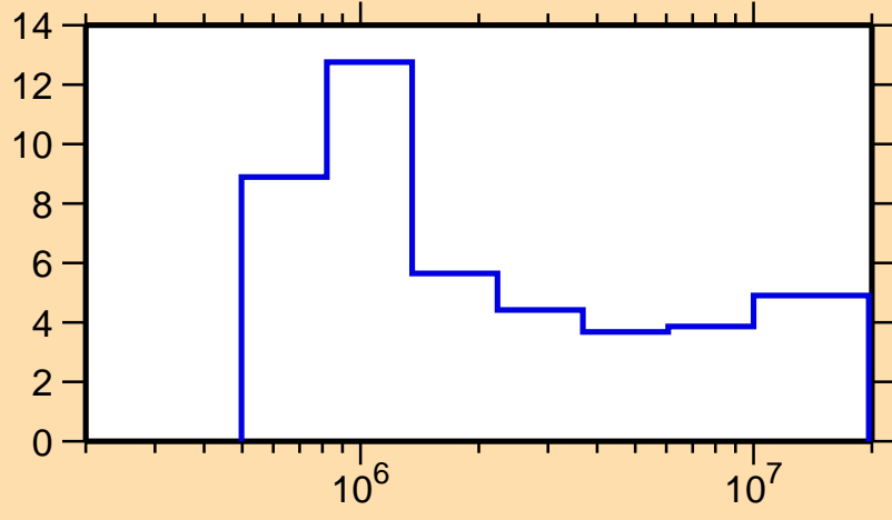
\Delta\sigma/\sigma vs. E for ^{32}\text{Si}(n,\text{nonel.})
