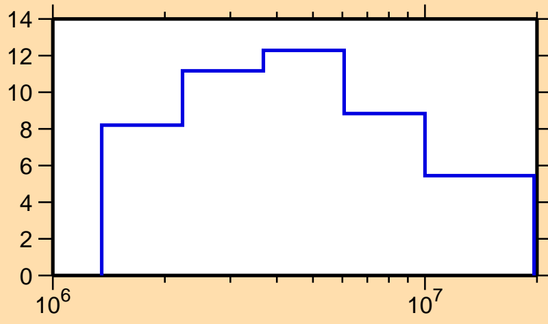
\Delta\sigma/\sigma vs. E for ^{32}\text{Si}(n,\text{el.})
