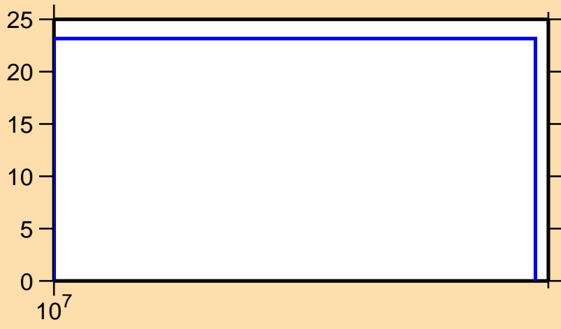
\Delta\sigma/\sigma vs. E for ^{32}\text{Si}(n,ncont.)
