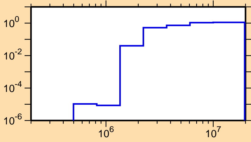
\sigma vs. E for ^{32}\text{Si}(n,\text{nonel.})
