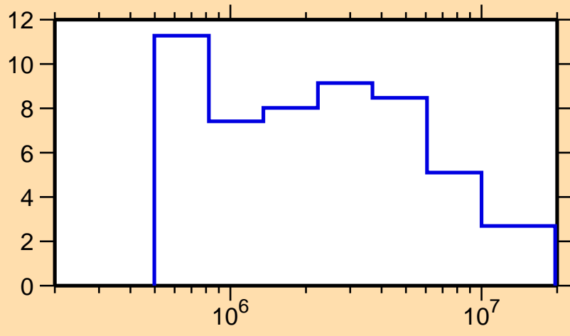
\Delta\sigma/\sigma vs. E for ^{32}\text{Si}(n,\text{tot.})
