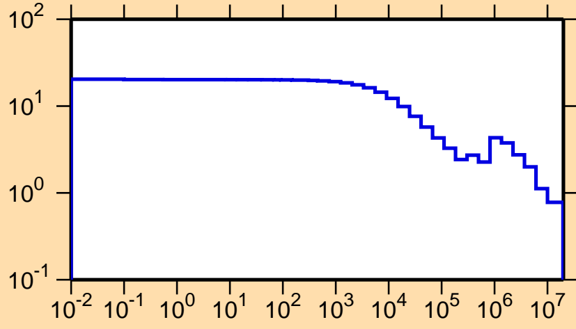
\sigma vs. E for ^{32}\text{Si}(n,\text{el.})
