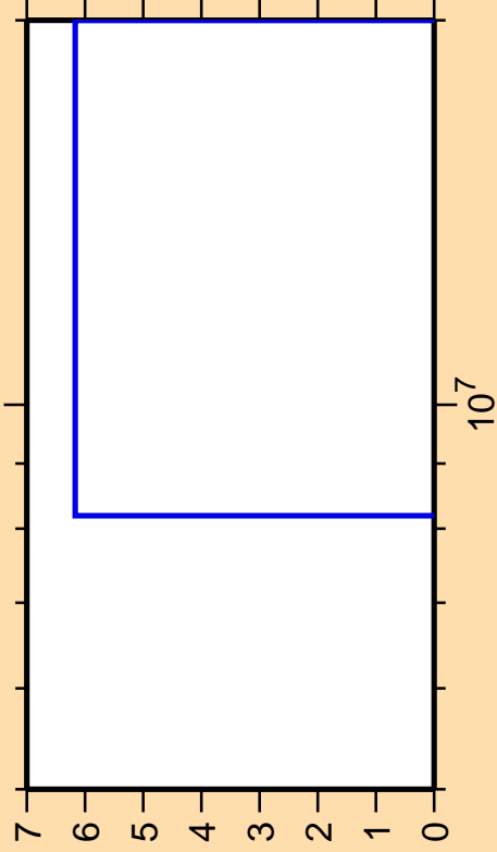
\Delta\sigma/\sigma vs. E for ^{32}\text{Si}(n,2n)
