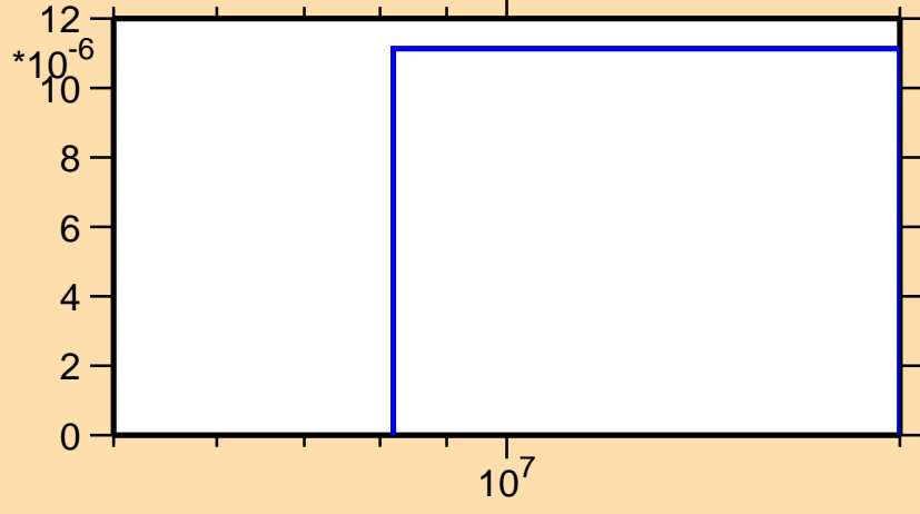
\sigma vs. E for ^{32}\text{Si}(n,d)
