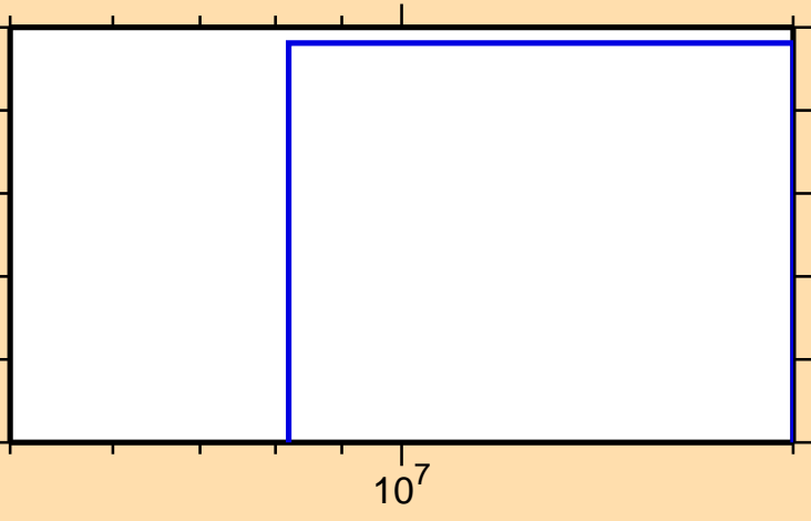
\sigma vs. E for ^{32}\text{Si}(n,n\alpha)
