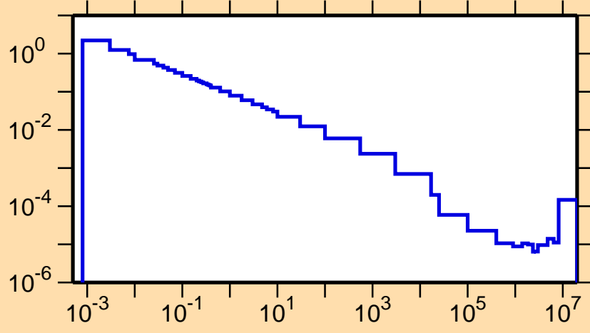
\sigma vs. E for ^{32}\text{Si}(n,\gamma)
