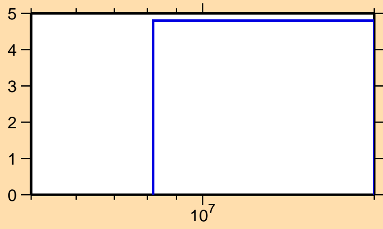
\Delta\sigma/\sigma vs. E for ^{32}\text{Si}(n,n\text{onel.})
