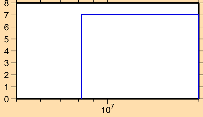
\Delta\sigma/\sigma vs. E for ^{32}\text{Si}(n,\text{inel.})
