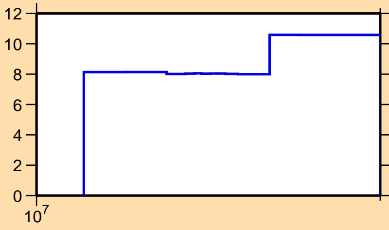
\Delta\sigma/\sigma vs. E for ^{33}\text{Si}(n,el.)
