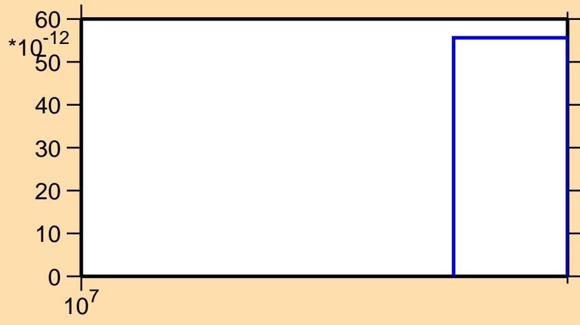
\sigma vs. E for ^{33}\text{Si}(n,\text{nd})
