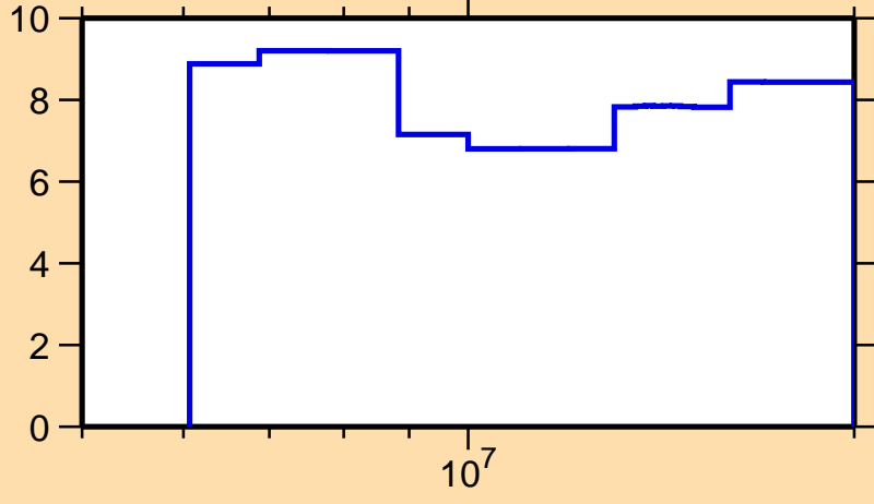
\Delta\sigma/\sigma vs. E for ^{33}\text{Si}(n,n\text{onel.})
