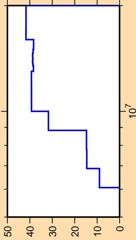
\Delta\sigma/\sigma vs. E for ^{33}\text{Si}(n,n_1)
