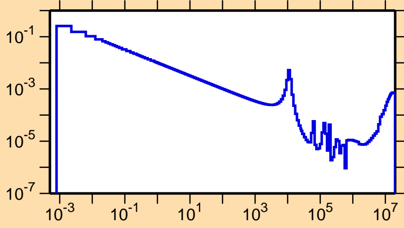
\sigma vs. E for ^{33}\text{Si}(n,\gamma)
