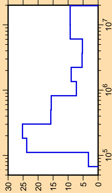
\Delta\mu/\mu vs. E for ^{33}\text{Si}(\text{mt251})
