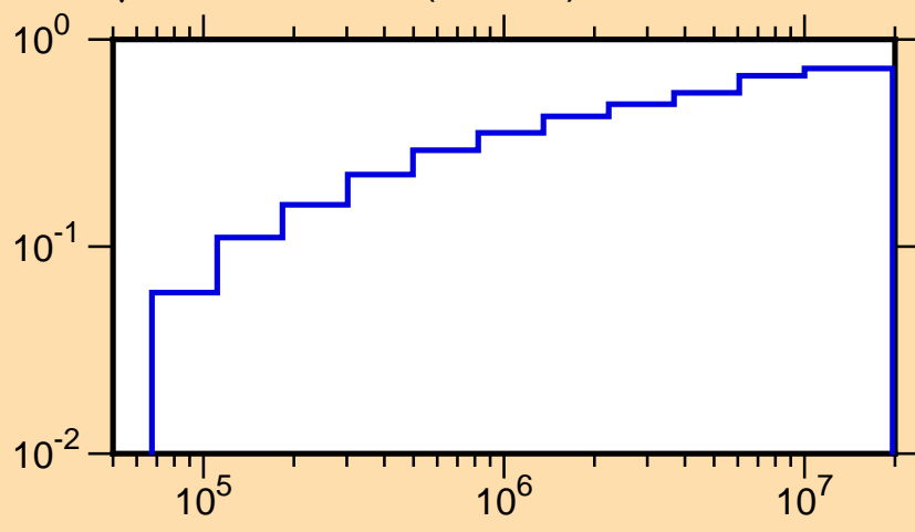
\mu vs. E for ^{33}\text{Si}(\text{mt251})
