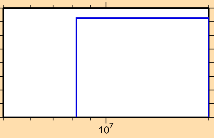
\sigma vs. E for ^{33}\text{Si}(n,n\alpha)
