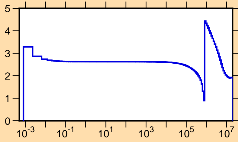
\sigma vs. E for ^{34}\text{Si}(n,\text{tot.})
