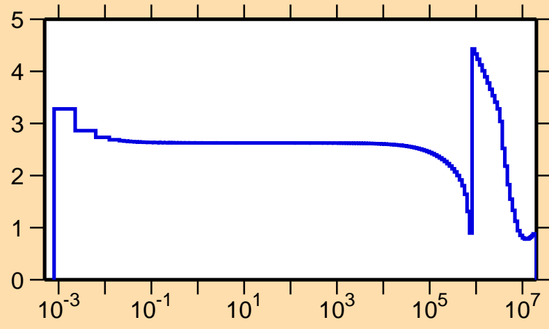
\sigma vs. E for ^{34}\text{Si}(n,\text{el.})
