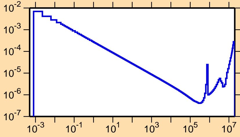
\sigma vs. E for ^{34}\text{Si}(n,\gamma)
