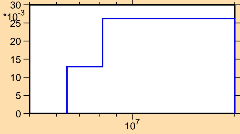
\sigma vs. E for ^{34}\text{Si}(n,n\text{cont.})
