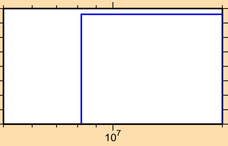
\sigma vs. E for ^{34}\text{Si}(n,\alpha)
