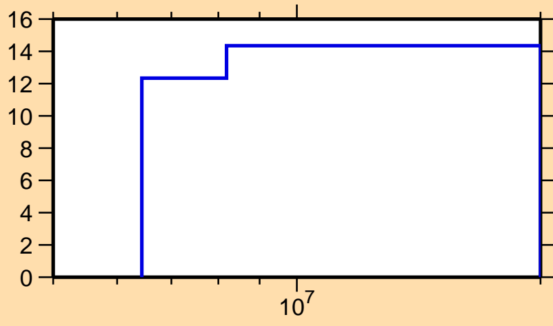
\Delta\sigma/\sigma vs. E for ^{34}\text{Si}(n,n\text{onel.})
