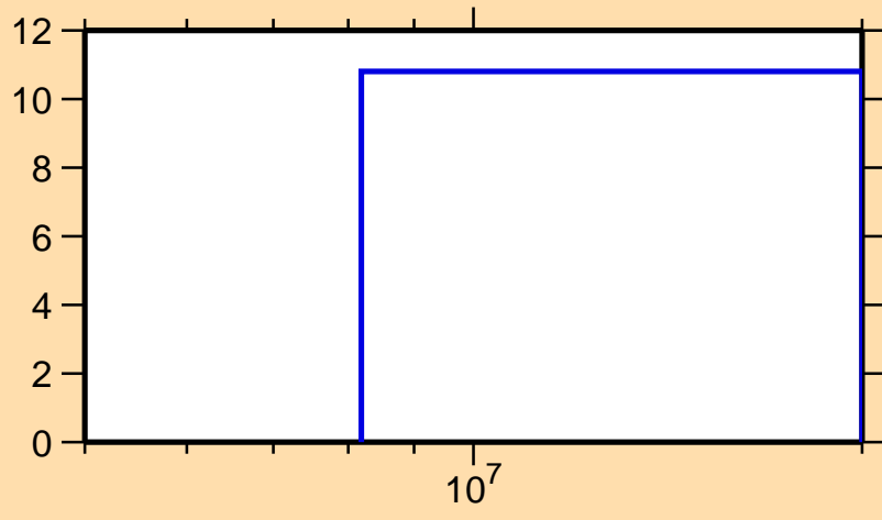
\Delta\sigma/\sigma vs. E for ^{34}\text{Si}(n,el.)
