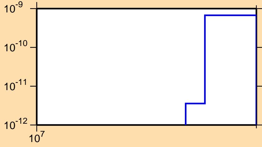
\sigma vs. E for ^{130}\text{Sm}(n,\text{nd})
