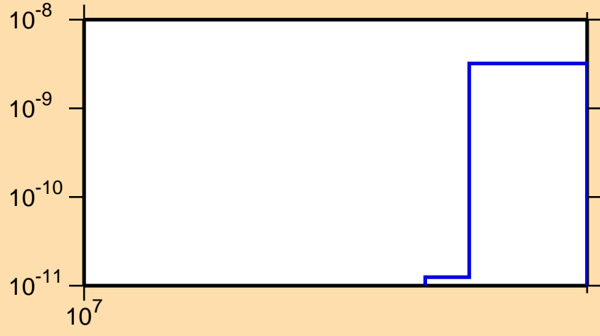
\sigma vs. E for ^{130}\text{Sm}(n,2n\alpha)
