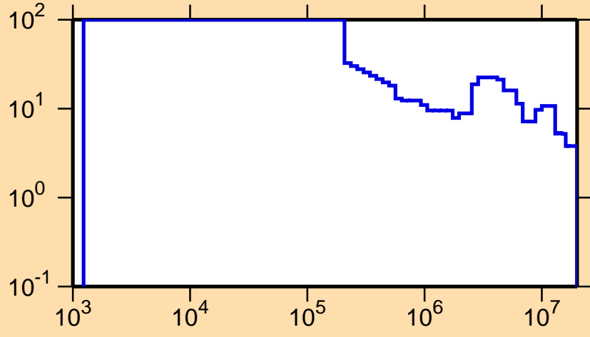
\Delta\sigma/\sigma vs. E for ^{130}\text{Sm}(n,el.)
