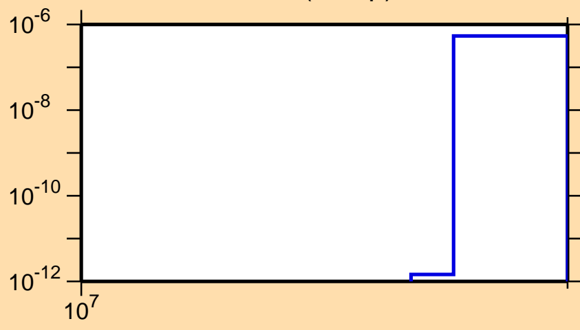
\sigma vs. E for ^{130}\text{Sm}(n,2np)
