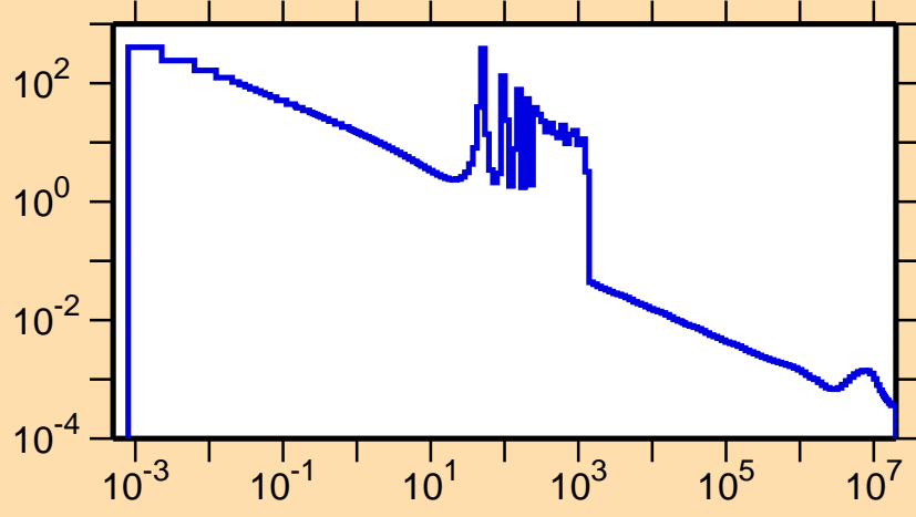
\sigma vs. E for ^{130}\text{Sm}(n,\gamma)
