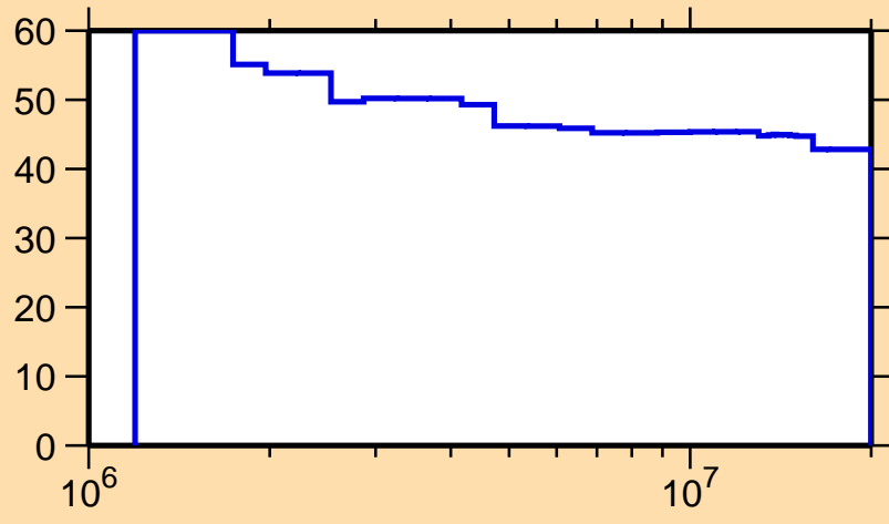
\Delta\sigma/\sigma vs. E for ^{130}\text{Sm}(n,ncont.)
