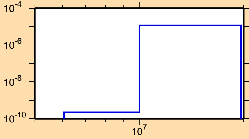
\sigma vs. E for ^{130}\text{Sm} (mt 45)
