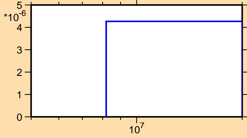
\sigma vs. E for ^{130}\text{Sm}(n,\text{pt})
