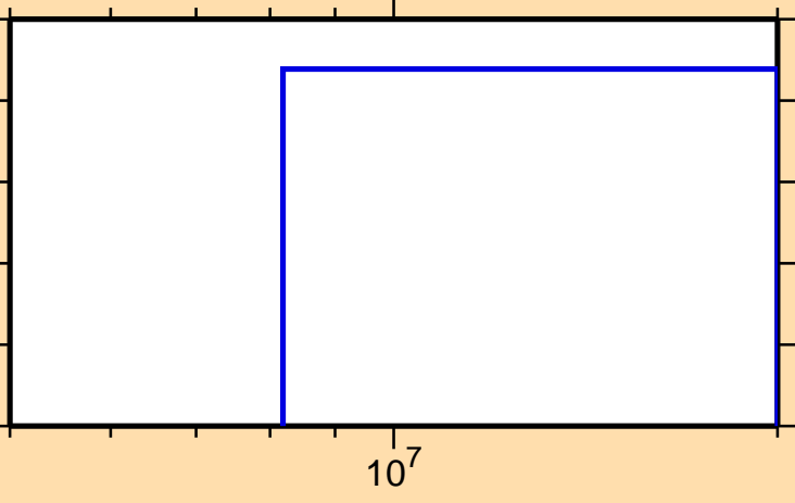
\sigma vs. E for ^{130}\text{Sm}(n,2np)
