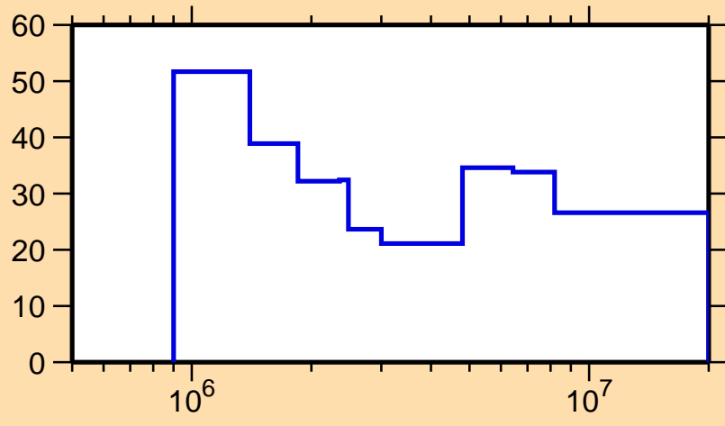
\Delta\sigma/\sigma vs. E for ^{130}\text{Sm}(n,n_1)
