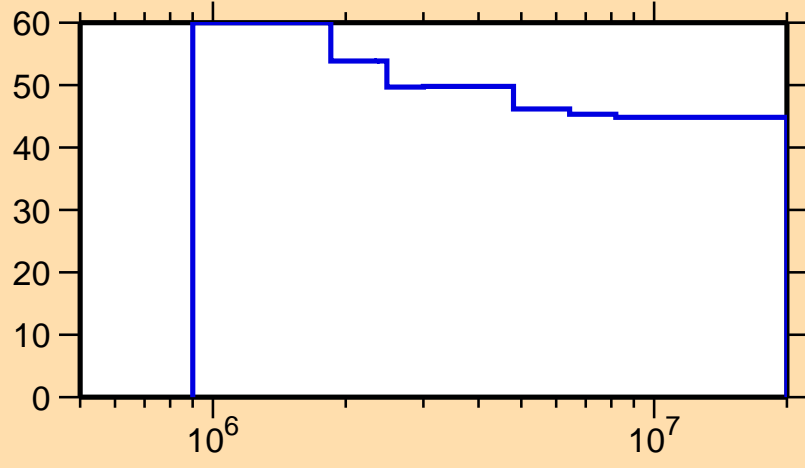
\Delta\sigma/\sigma vs. E for ^{130}\text{Sm}(n,n\text{cont.})
