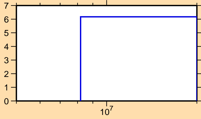
\Delta\sigma/\sigma vs. E for ^{130}\text{Sm}(n,\text{el.})
