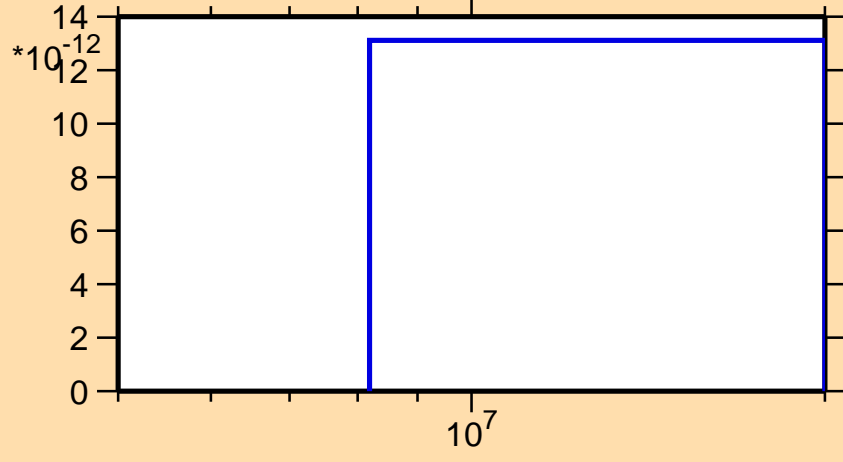
\sigma vs. E for ^{130}\text{Sm} (mt 34)
