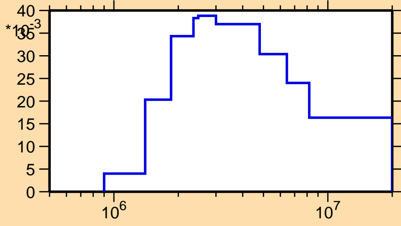
\sigma vs. E for ^{130}\text{Sm}(n,n_2)
