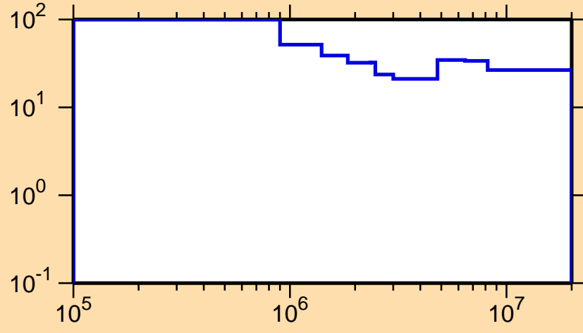
\Delta\sigma/\sigma vs. E for ^{130}\text{Sm}(n,n_1)
