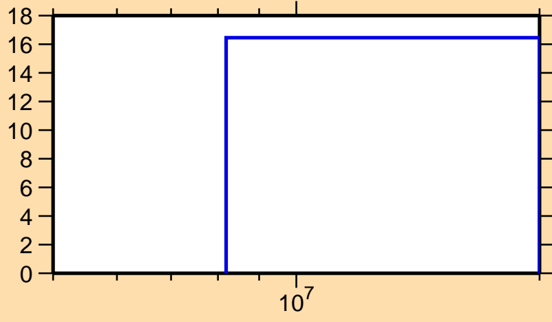
\Delta\sigma/\sigma vs. E for ^{130}\text{Sm}(n,\text{inel.})
