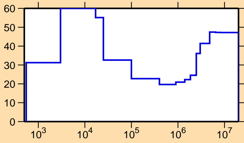
\Delta\sigma/\sigma vs. E for ^{130}\text{Sm}(n,p)
