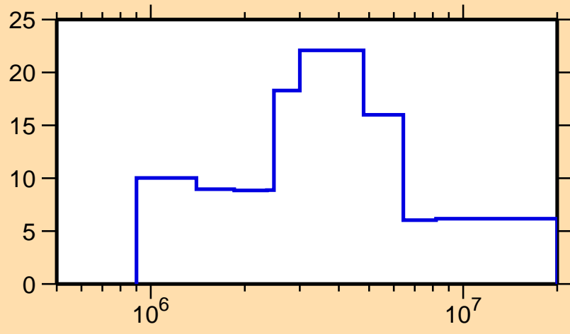
\Delta\sigma/\sigma vs. E for ^{130}\text{Sm}(n, el.)
