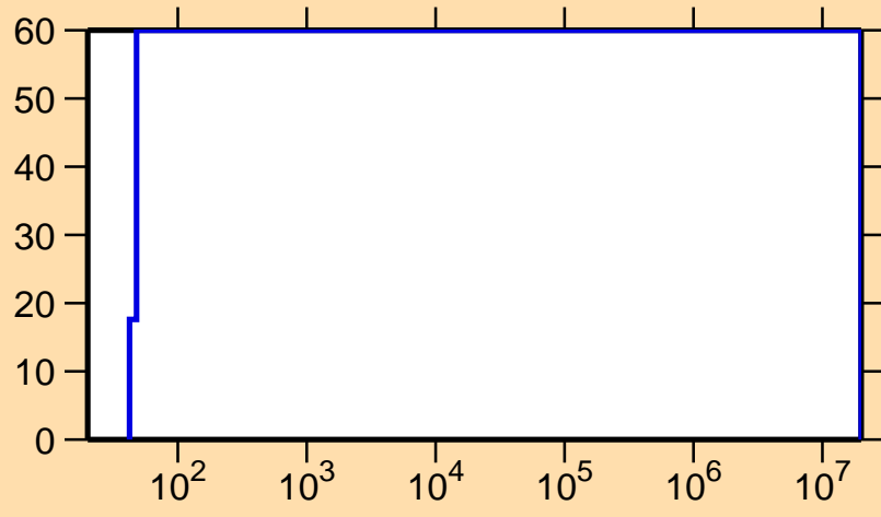
\Delta\sigma/\sigma vs. E for ^{131}\text{Sm}(n,\gamma)
