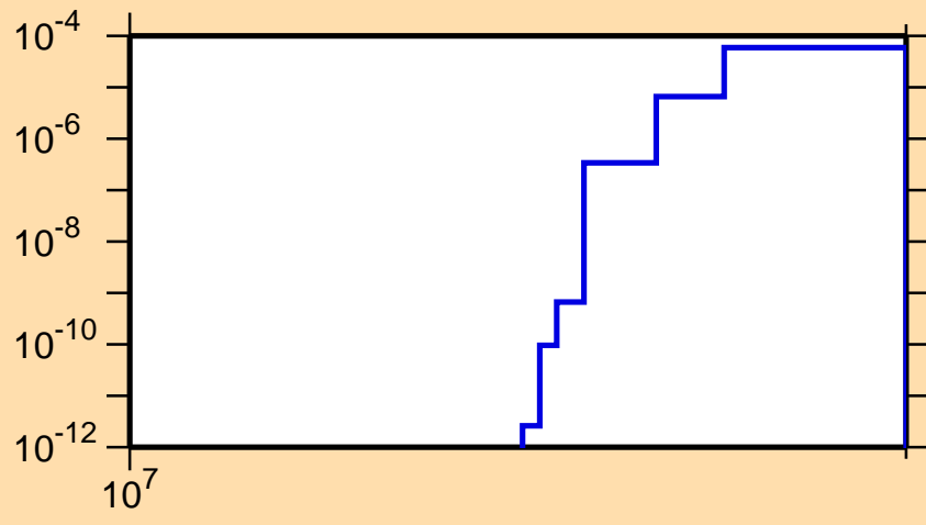
\sigma vs. E for ^{131}\text{Sm}(n,2np)
