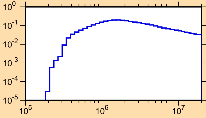
\sigma vs. E for ^{131}\text{Sm}(n,n_1)
