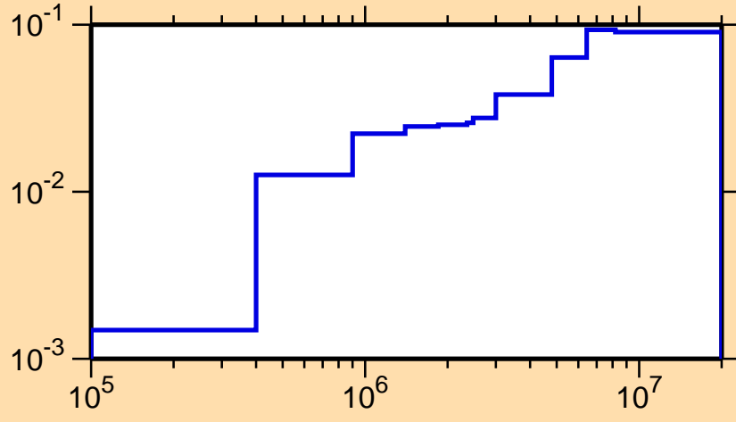
\sigma vs. E for ^{131}\text{Sm}(n,n\text{cont.})
