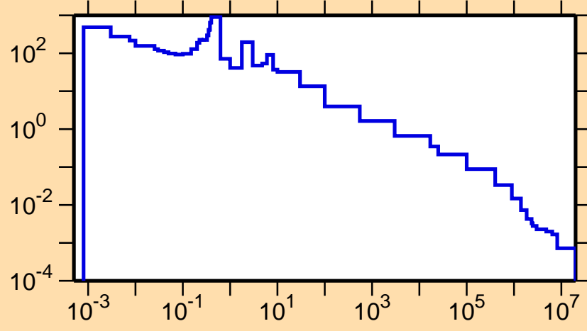
\sigma vs. E for ^{131}\text{Sm}(n,\gamma)
