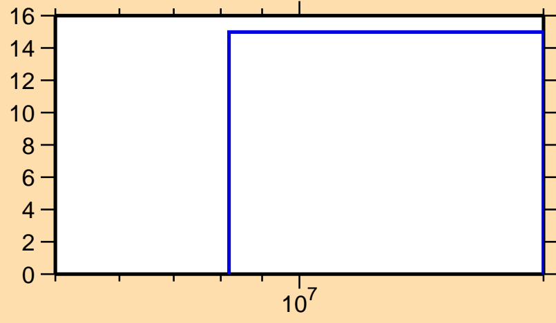
\Delta\sigma/\sigma vs. E for ^{131}\text{Sm}(n,\text{nonel.})
