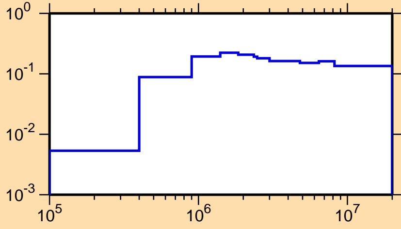
\sigma vs. E for ^{131}\text{Sm}(n,\text{inel.})
