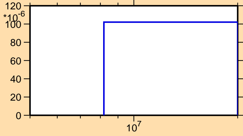
\sigma vs. E for ^{131}\text{Sm}(n,\text{pt})
