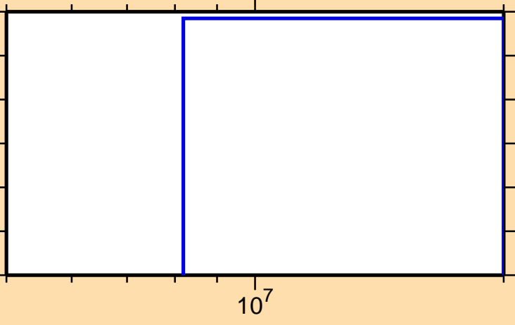
\sigma vs. E for ^{131}\text{Sm}(n,2n)
