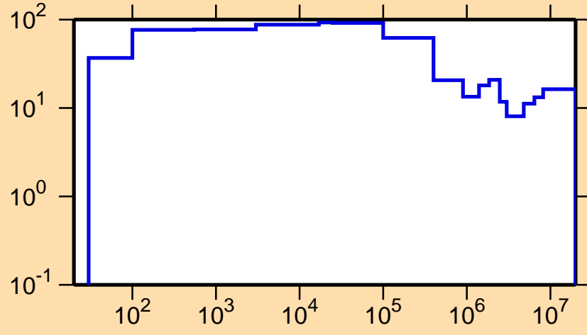
\Delta\sigma/\sigma vs. E for ^{131}\text{Sm}(n,el.)
