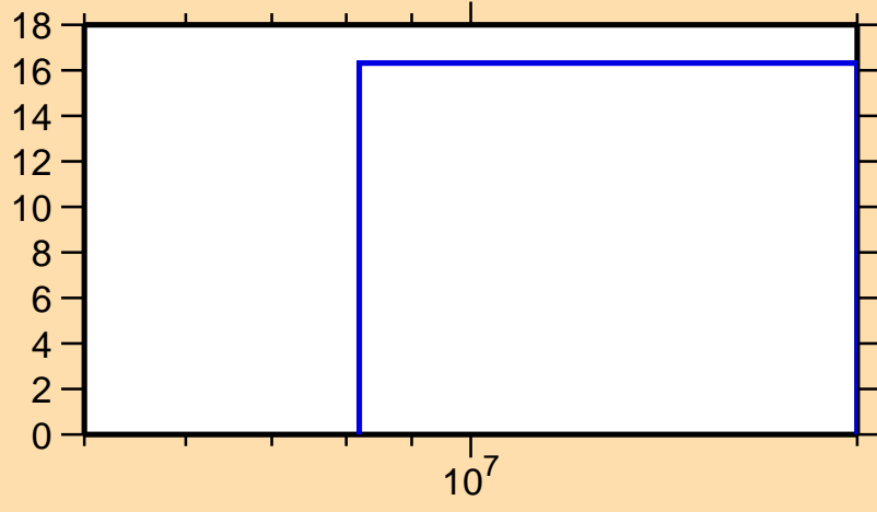
\Delta\sigma/\sigma vs. E for ^{131}\text{Sm}(n,\text{el.})
