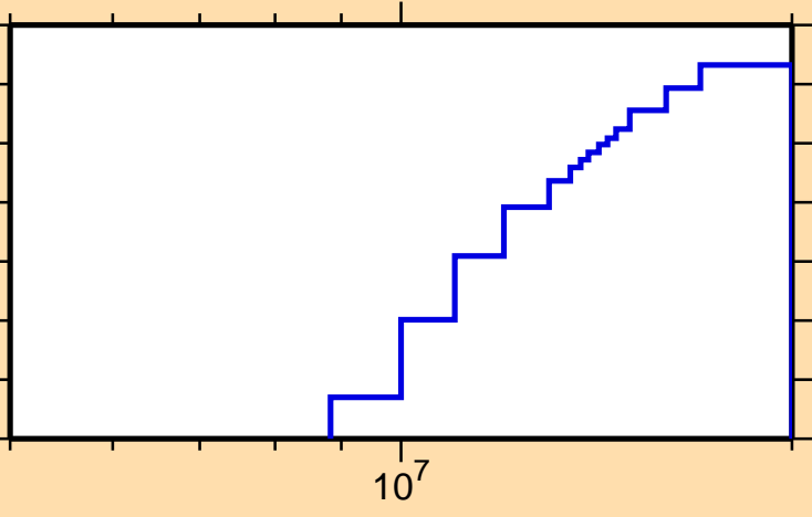
\sigma vs. E for ^{133}\text{Sm}(\text{mt117})
