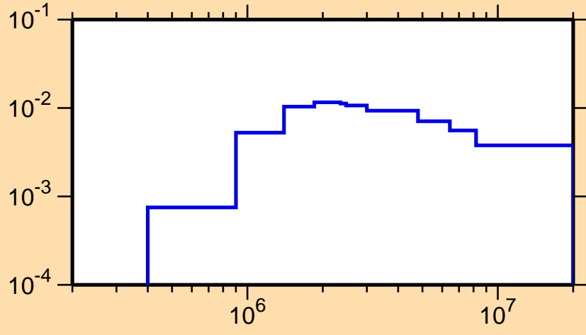
\sigma vs. E for ^{133}\text{Sm}(n,n_4)
