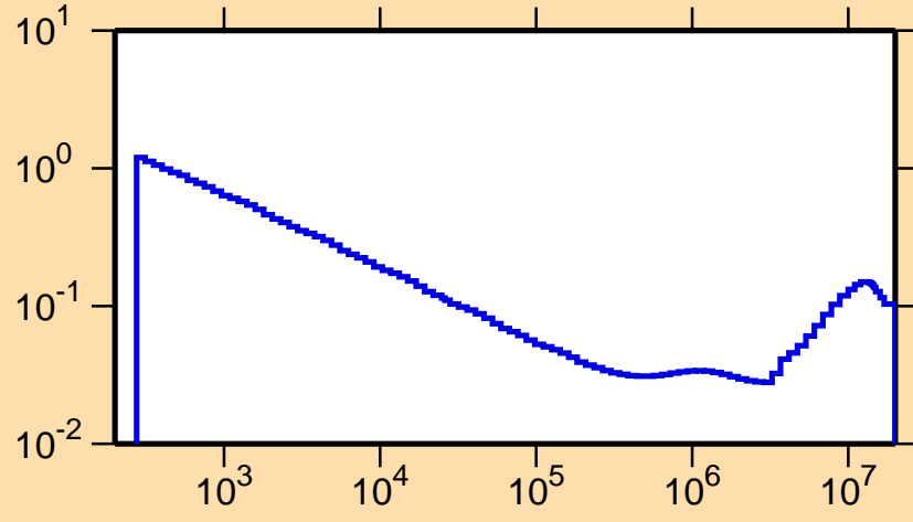
\sigma vs. E for ^{133}\text{Sm}(n,\alpha)
