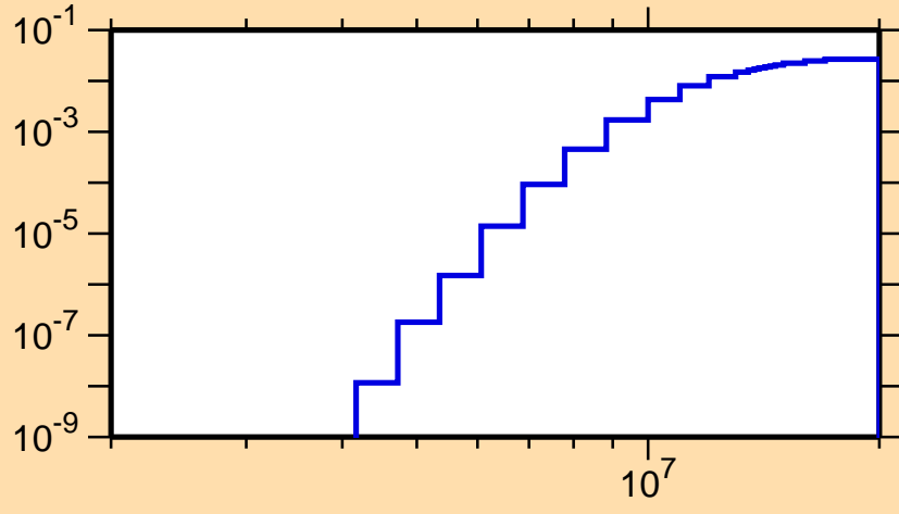
\sigma vs. E for ^{133}\text{Sm}(n,d)
