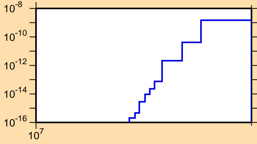
\sigma vs. E for ^{134}\text{Sm} (mt 34)
