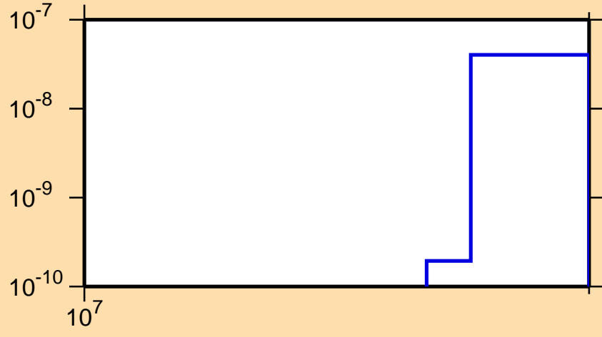
\sigma vs. E for ^{134}\text{Sm}(n,\text{nd})
