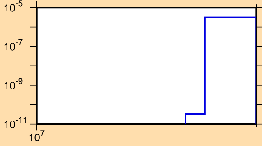
\sigma vs. E for ^{134}\text{Sm}(n,2np)
