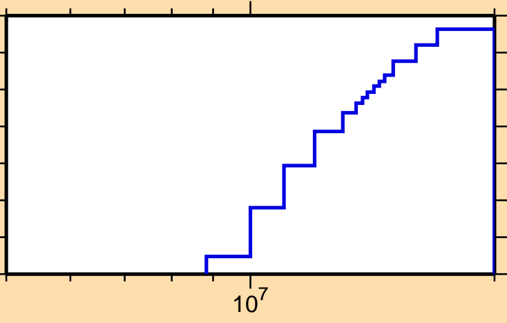
\sigma vs. E for ^{134}\text{Sm}(\text{mt117})
