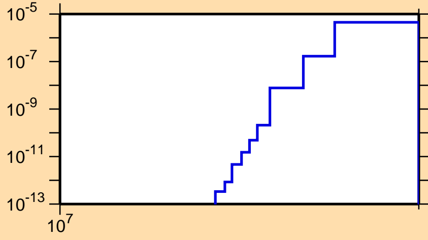
\sigma vs. E for ^{134}\text{Sm}(n,\text{pt})
