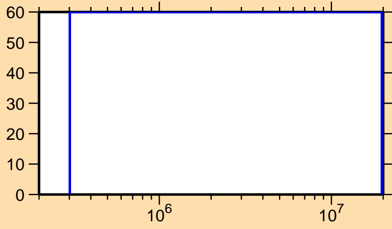
\Delta\sigma/\sigma vs. E for ^{134}\text{Sm}(n,n\text{cont.})
